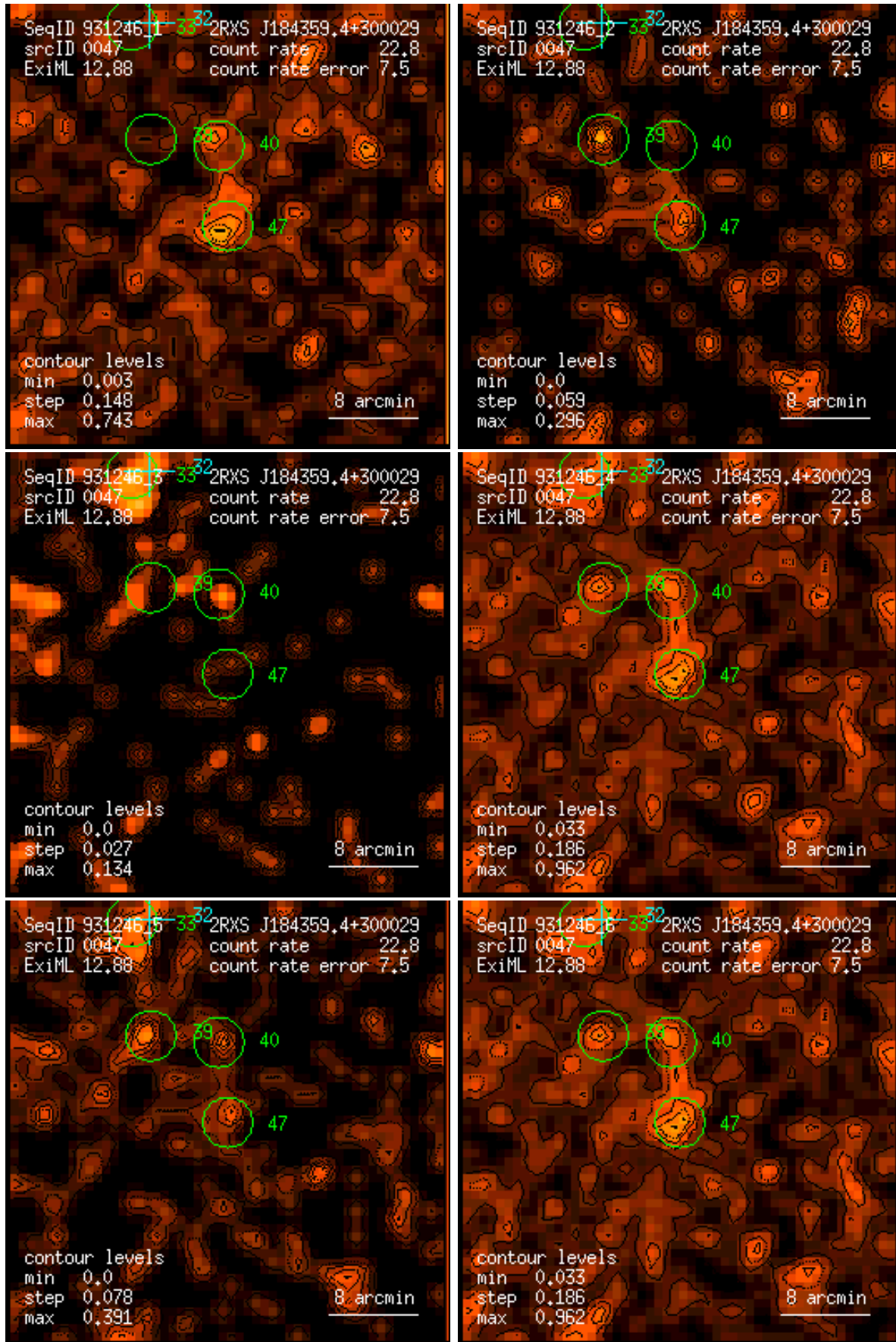
Figure 47: RASS 931246: detection 0047: band rate images, Gaussian filter: (1) PSPC channels 11 – 41, (2) 52 – 90, (3) 91 – 201, (4) 11 – 235, (5) 52 – 201, (6) 11 – 201. Broad band rates in counts/ks. Band rate contour levels in counts/ks/arcmin 2 .
