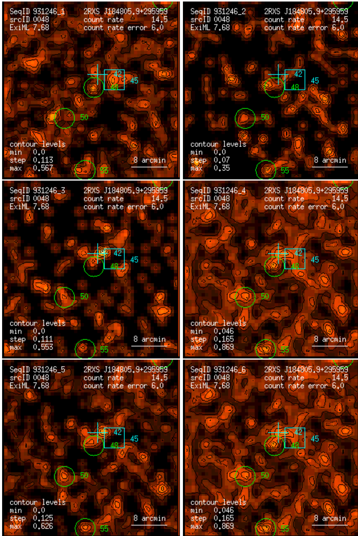
Figure 48: RASS 931246: detection 0048: band rate images, Gaussian filter: (1) PSPC channels 11 – 41, (2) 52 – 90, (3) 91 – 201, (4) 11 – 235, (5) 52 – 201, (6) 11 – 201. Broad band rates in counts/ks. Band rate contour levels in counts/ks/arcmin 2 .
