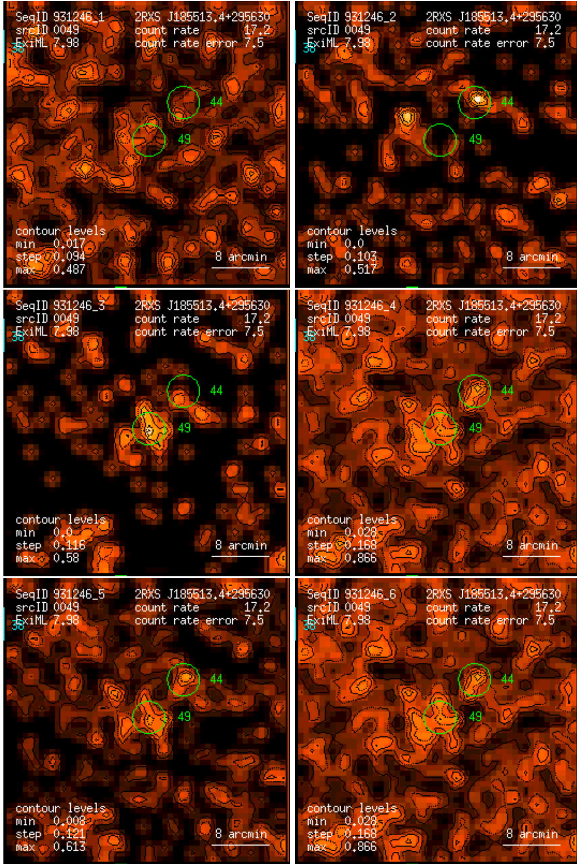
Figure 49: RASS 931246: detection 0049: band rate images, Gaussian filter: (1) PSPC channels 11 – 41, (2) 52 – 90, (3) 91 – 201, (4) 11 – 235, (5) 52 – 201, (6) 11 – 201. Broad band rates in counts/ks. Band rate contour levels in counts/ks/arcmin 2 .
