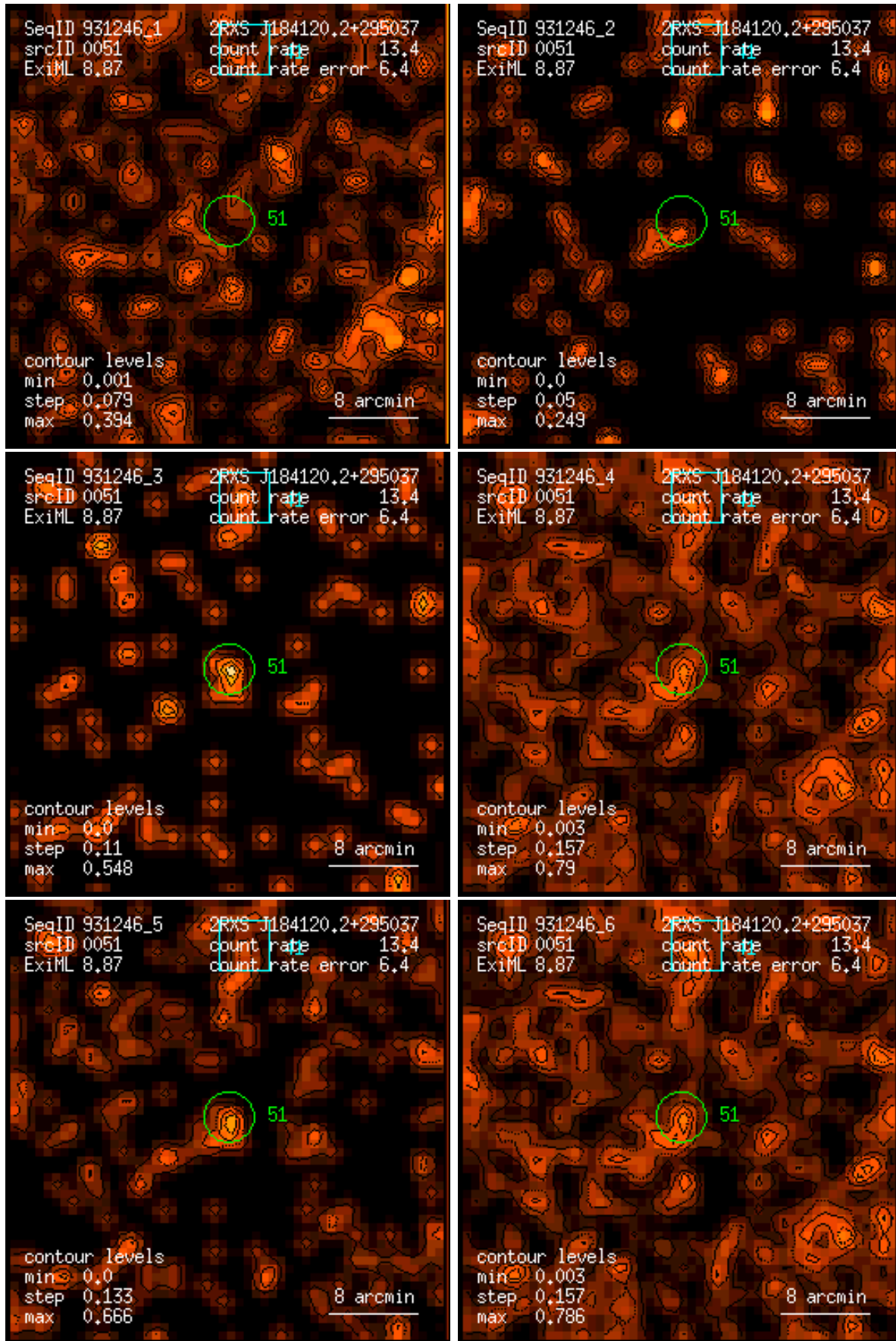
Figure 51: RASS 931246: detection 0051: band rate images, Gaussian filter: (1) PSPC channels 11 – 41, (2) 52 – 90, (3) 91 – 201, (4) 11 – 235, (5) 52 – 201, (6) 11 – 201. Broad band rates in counts/ks. Band rate contour levels in counts/ks/arcmin 2 .
