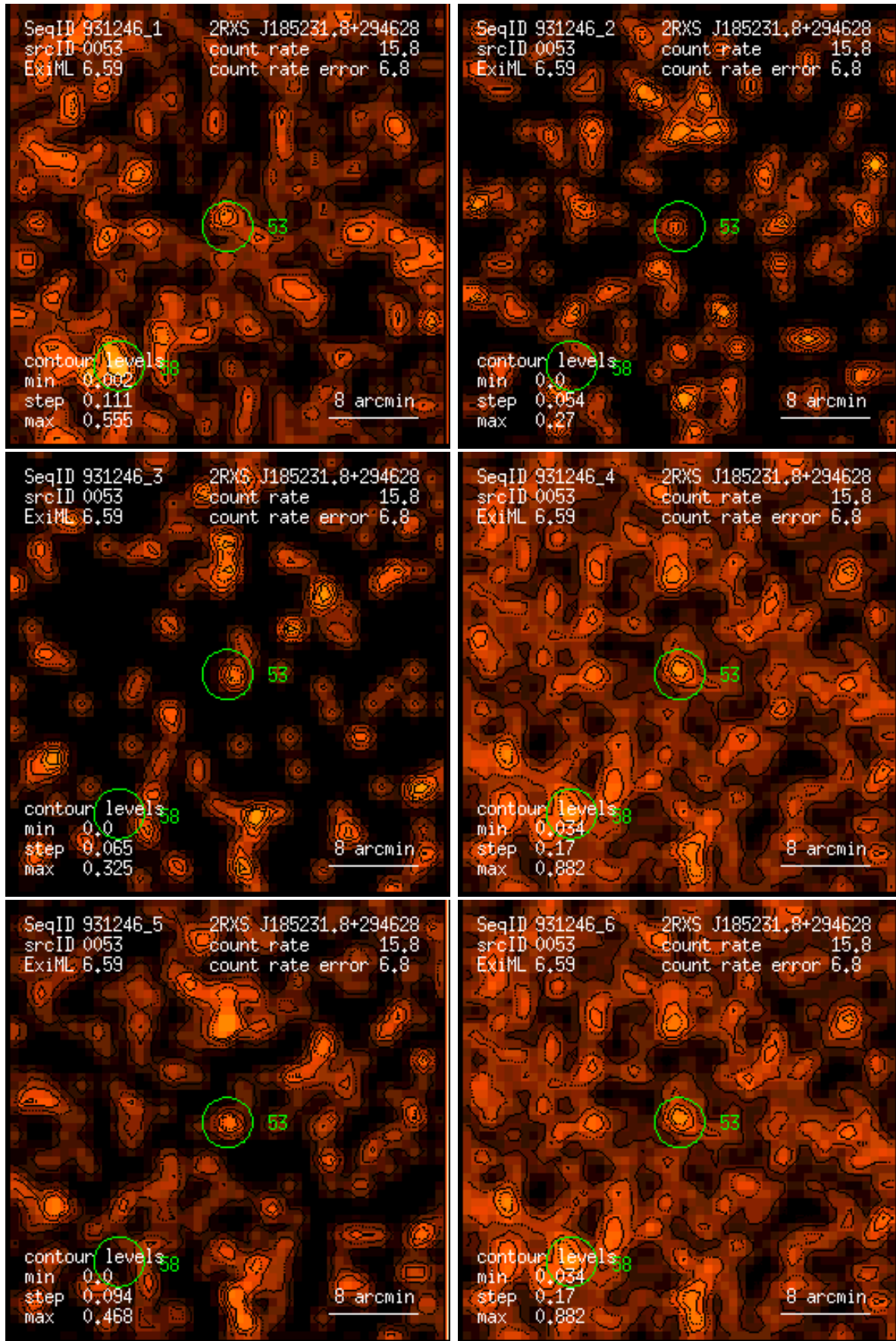
Figure 53: RASS 931246: detection 0053: band rate images, Gaussian filter: (1) PSPC channels 11 – 41, (2) 52 – 90, (3) 91 – 201, (4) 11 – 235, (5) 52 – 201, (6) 11 – 201. Broad band rates in counts/ks. Band rate contour levels in counts/ks/arcmin 2 .
