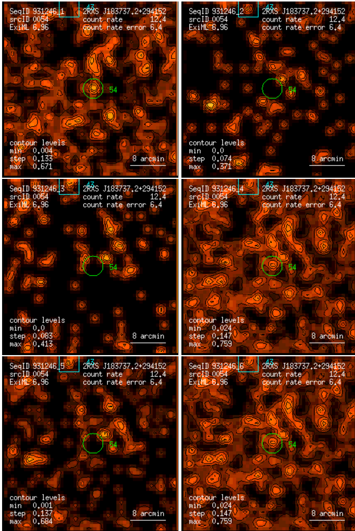
Figure 54: RASS 931246: detection 0054: band rate images, Gaussian filter: (1) PSPC channels 11 – 41, (2) 52 – 90, (3) 91 – 201, (4) 11 – 235, (5) 52 – 201, (6) 11 – 201. Broad band rates in counts/ks. Band rate contour levels in counts/ks/arcmin 2 .
