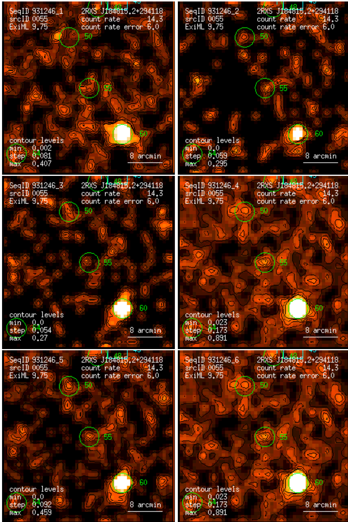
Figure 55: RASS 931246: detection 0055: band rate images, Gaussian filter: (1) PSPC channels 11 – 41, (2) 52 – 90, (3) 91 – 201, (4) 11 – 235, (5) 52 – 201, (6) 11 – 201. Broad band rates in counts/ks. Band rate contour levels in counts/ks/arcmin 2 .
