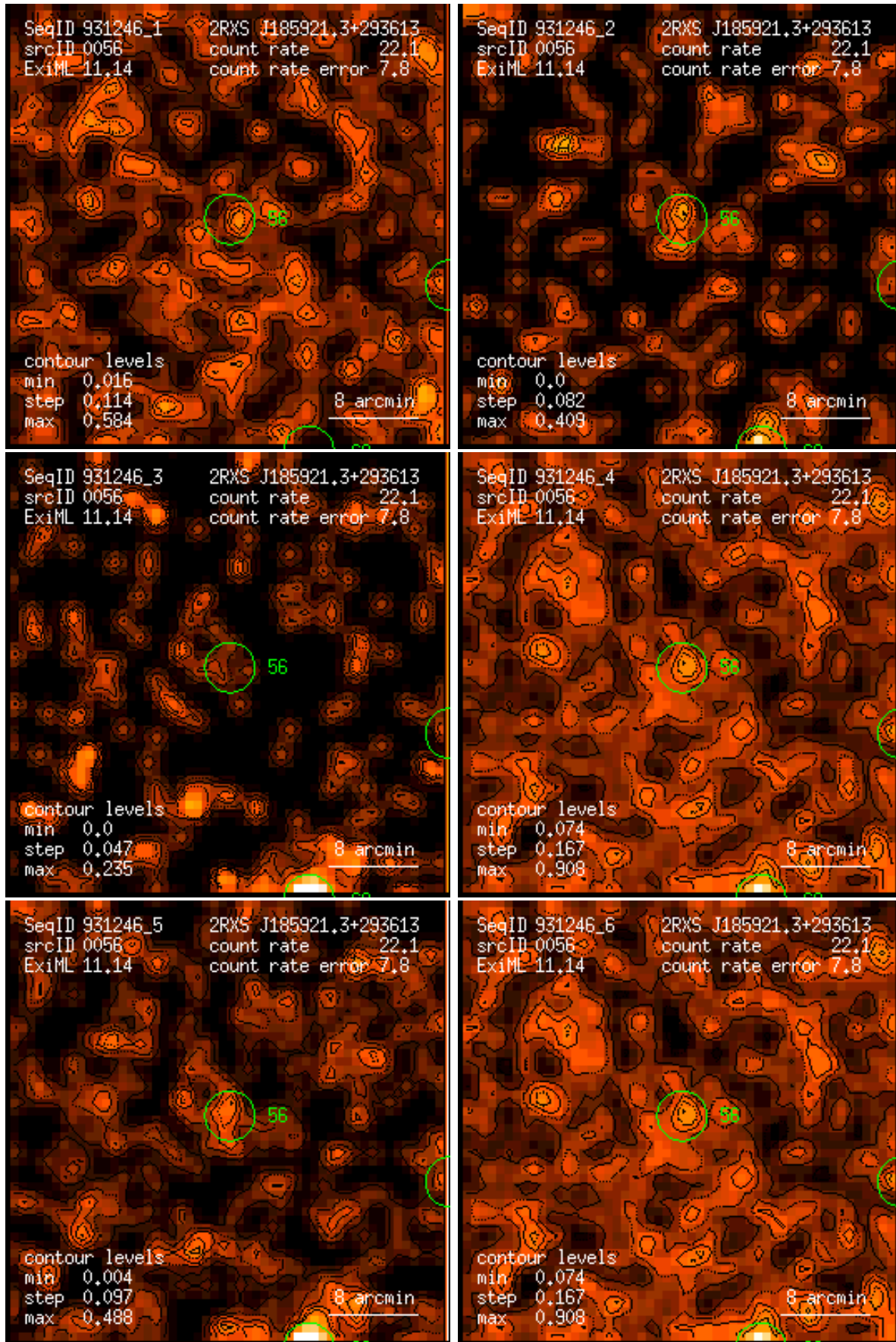
Figure 56: RASS 931246: detection 0056: band rate images, Gaussian filter: (1) PSPC channels 11 – 41, (2) 52 – 90, (3) 91 – 201, (4) 11 – 235, (5) 52 – 201, (6) 11 – 201. Broad band rates in counts/ks. Band rate contour levels in counts/ks/arcmin 2 .
