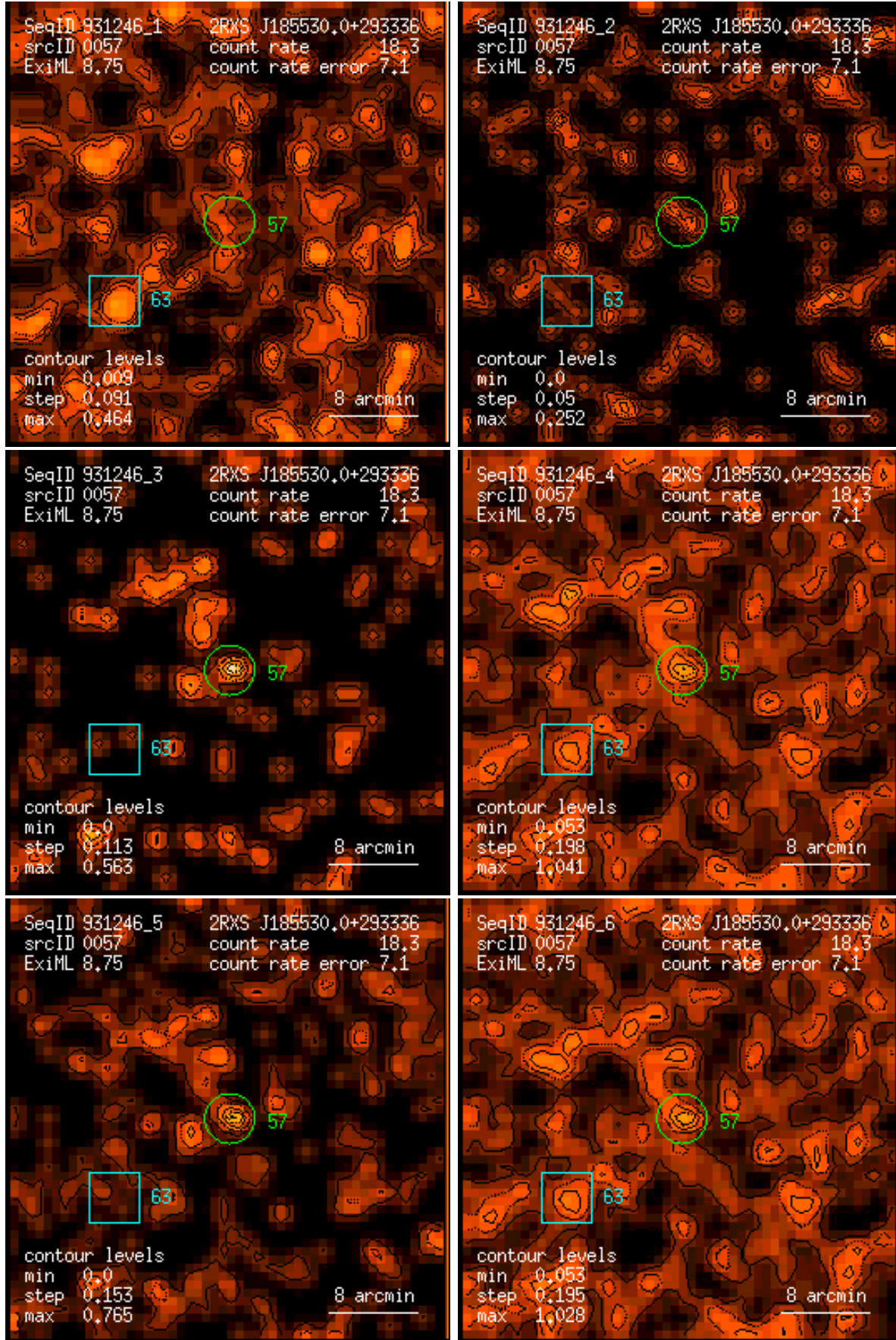
Figure 57: RASS 931246: detection 0057: band rate images, Gaussian filter: (1) PSPC channels 11 – 41, (2) 52 – 90, (3) 91 – 201, (4) 11 – 235, (5) 52 – 201, (6) 11 – 201. Broad band rates in counts/ks. Band rate contour levels in counts/ks/arcmin 2 .
