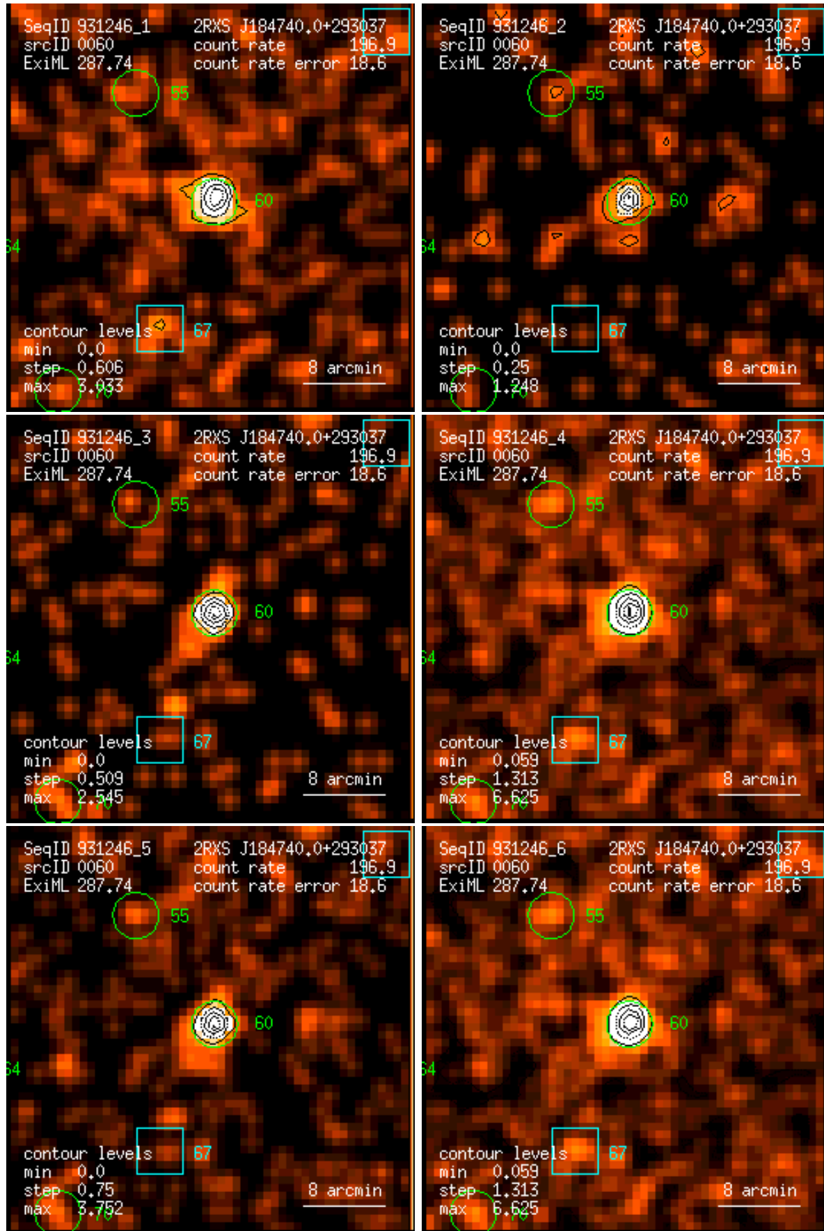
Figure 60: RASS 931246: detection 0060: band rate images, Gaussian filter: (1) PSPC channels 11 – 41, (2) 52 – 90, (3) 91 – 201, (4) 11 – 235, (5) 52 – 201, (6) 11 – 201. Broad band rates in counts/ks. Band rate contour levels in counts/ks/arcmin 2 .
