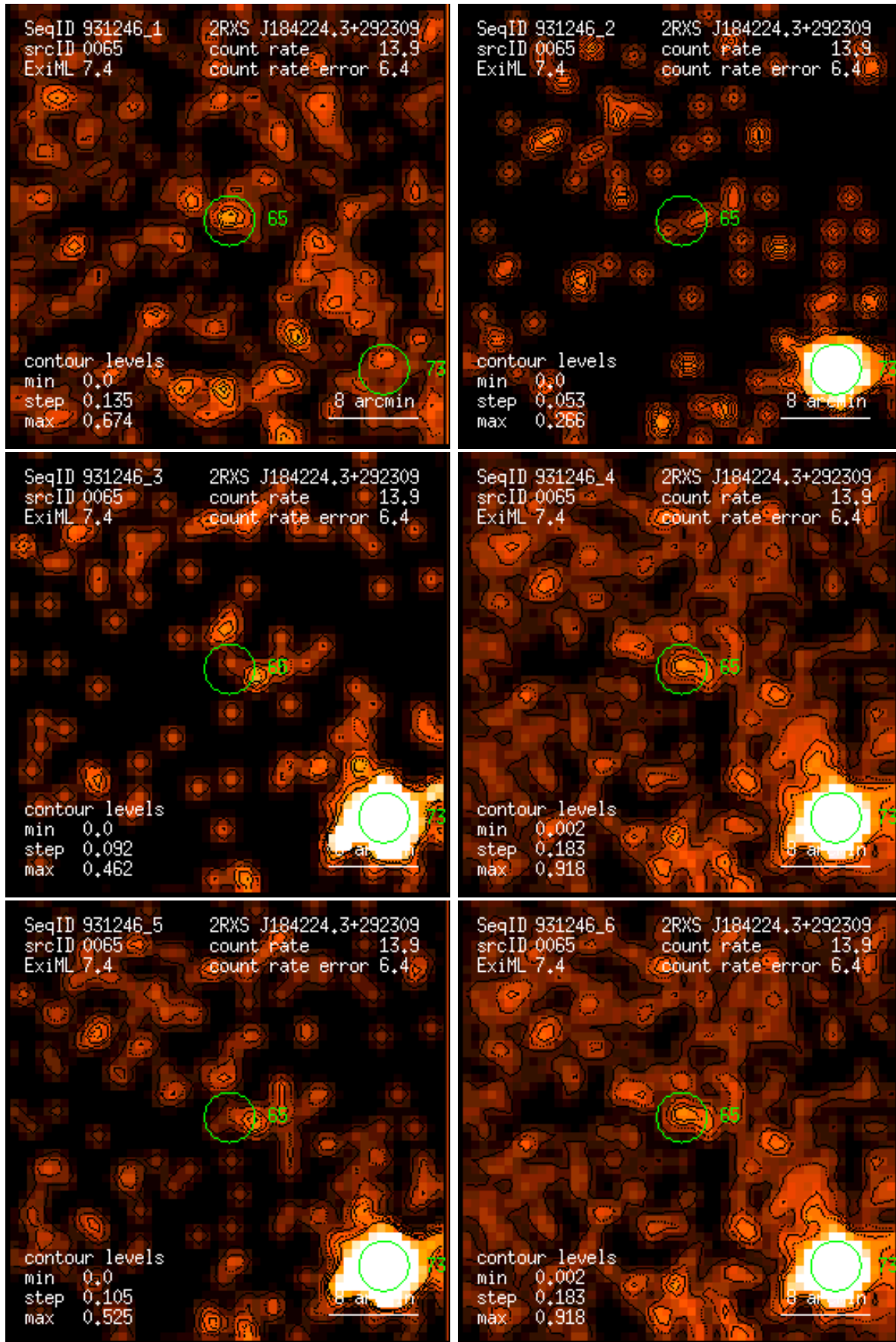
Figure 65: RASS 931246: detection 0065: band rate images, Gaussian filter: (1) PSPC channels 11 – 41, (2) 52 – 90, (3) 91 – 201, (4) 11 – 235, (5) 52 – 201, (6) 11 – 201. Broad band rates in counts/ks. Band rate contour levels in counts/ks/arcmin 2 .
