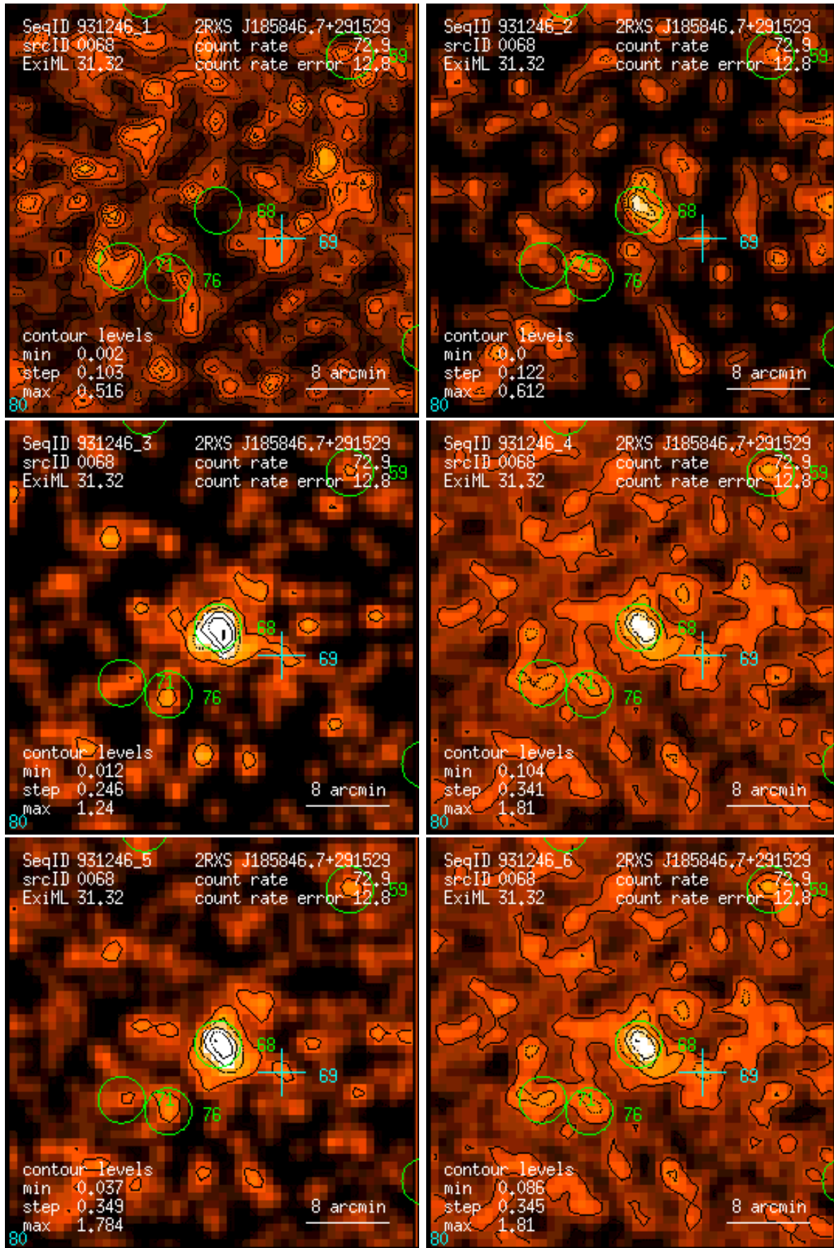
Figure 68: RASS 931246: detection 0068: band rate images, Gaussian filter: (1) PSPC channels 11 – 41, (2) 52 – 90, (3) 91 – 201, (4) 11 – 235, (5) 52 – 201, (6) 11 – 201. Broad band rates in counts/ks. Band rate contour levels in counts/ks/arcmin 2 .
