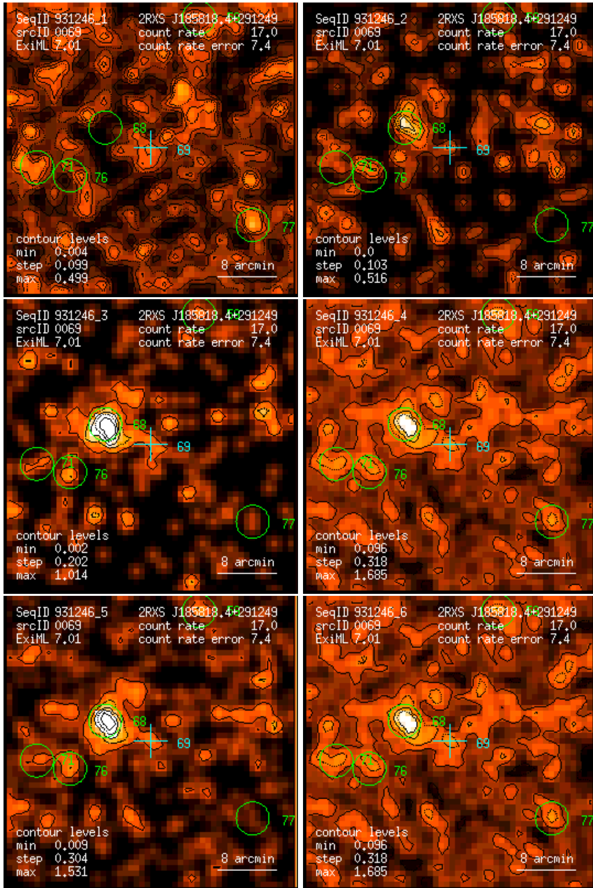
Figure 69: RASS 931246: detection 0069: band rate images, Gaussian filter: (1) PSPC channels 11 – 41, (2) 52 – 90, (3) 91 – 201, (4) 11 – 235, (5) 52 – 201, (6) 11 – 201. Broad band rates in counts/ks. Band rate contour levels in counts/ks/arcmin 2 .
