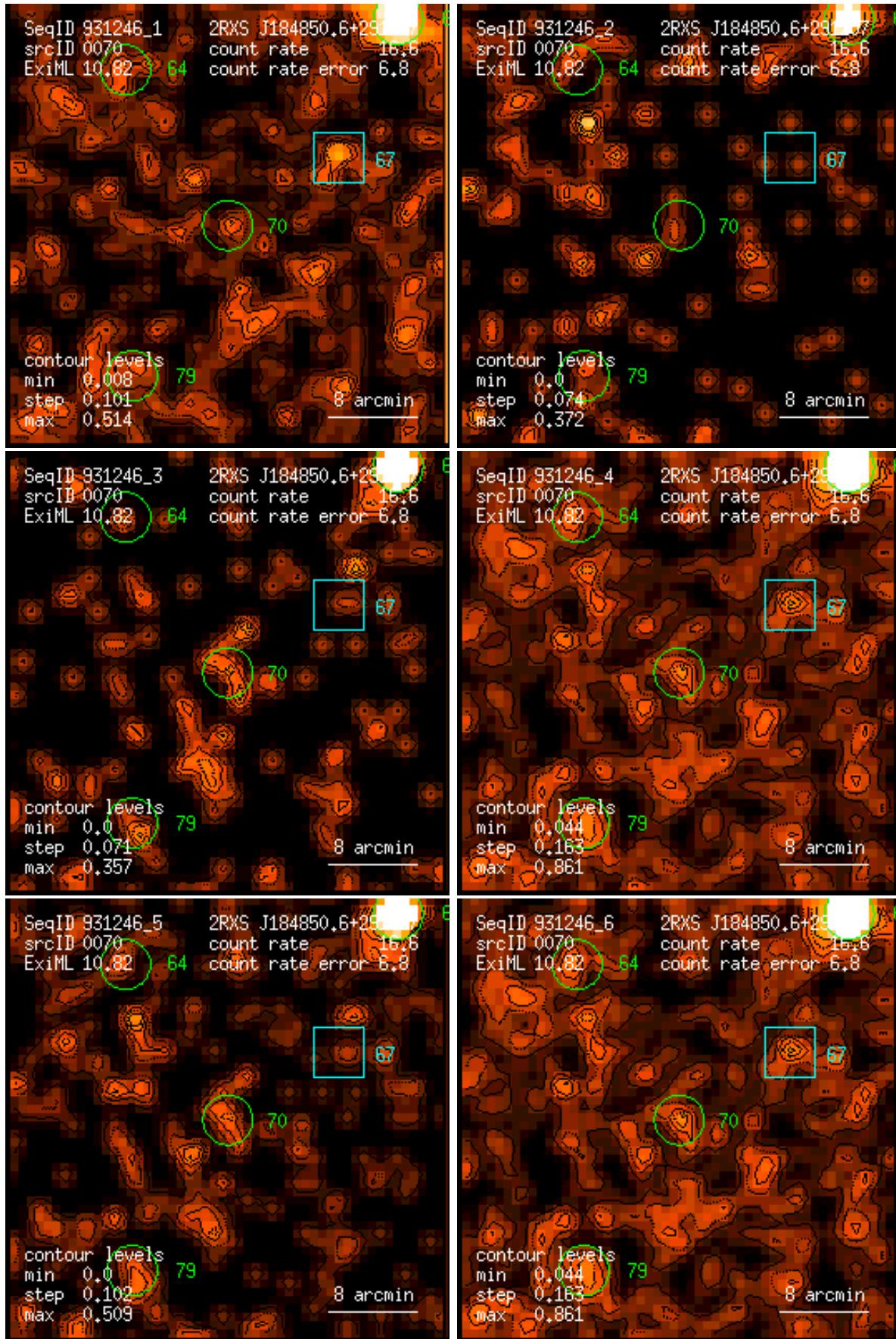
Figure 70: RASS 931246: detection 0070: band rate images, Gaussian filter: (1) PSPC channels 11 – 41, (2) 52 – 90, (3) 91 – 201, (4) 11 – 235, (5) 52 – 201, (6) 11 – 201. Broad band rates in counts/ks. Band rate contour levels in counts/ks/arcmin 2 .
