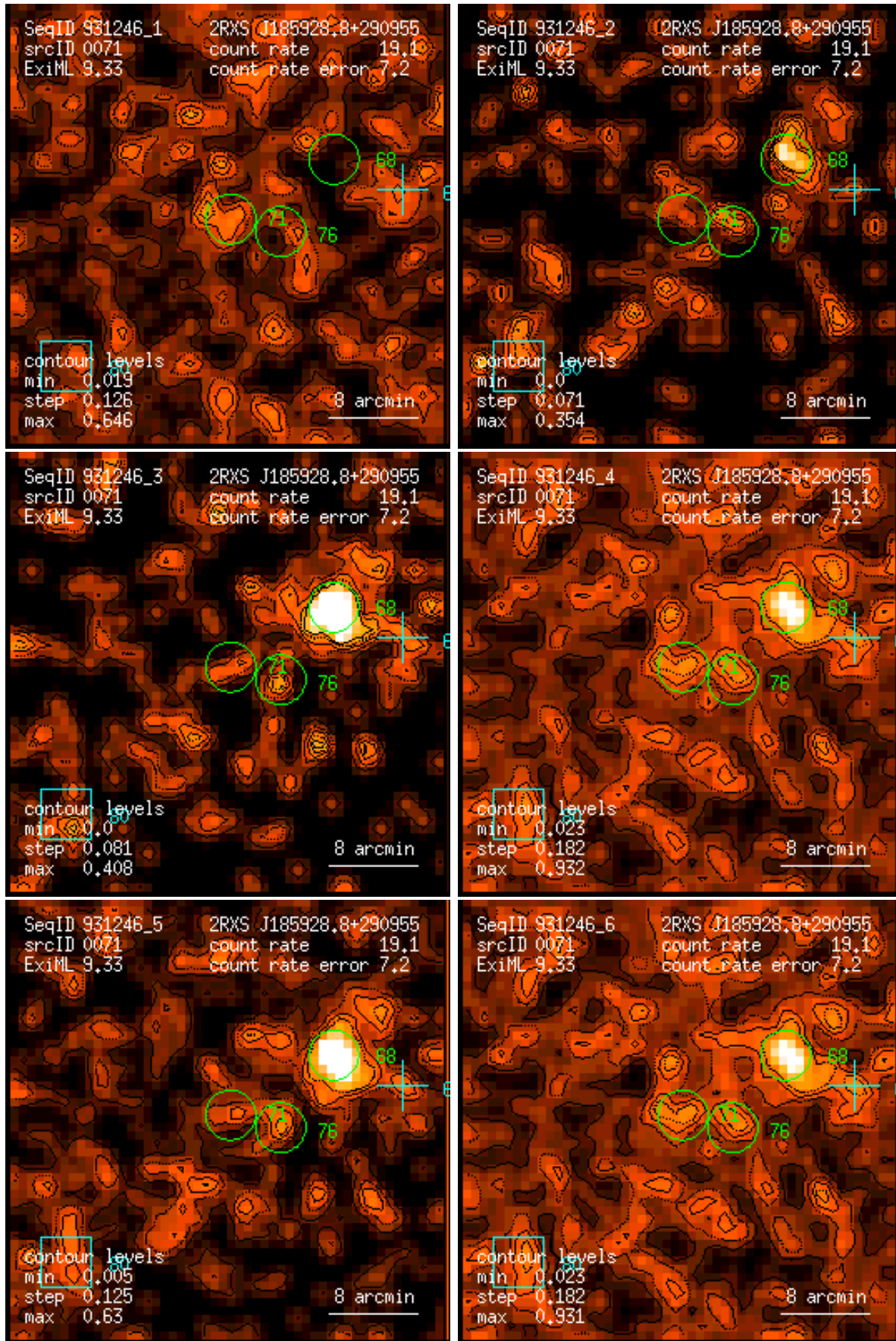
Figure 71: RASS 931246: detection 0071: band rate images, Gaussian filter: (1) PSPC channels 11 – 41, (2) 52 – 90, (3) 91 – 201, (4) 11 – 235, (5) 52 – 201, (6) 11 – 201. Broad band rates in counts/ks. Band rate contour levels in counts/ks/arcmin 2 .
