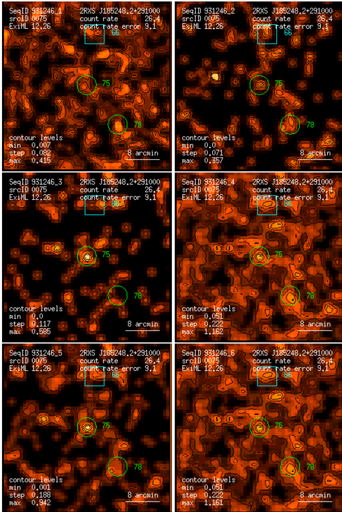
Figure 75: RASS 931246: detection 0075: band rate images, Gaussian filter: (1) PSPC channels 11 – 41, (2) 52 – 90, (3) 91 – 201, (4) 11 – 235, (5) 52 – 201, (6) 11 – 201. Broad band rates in counts/ks. Band rate contour levels in counts/ks/arcmin 2 .
