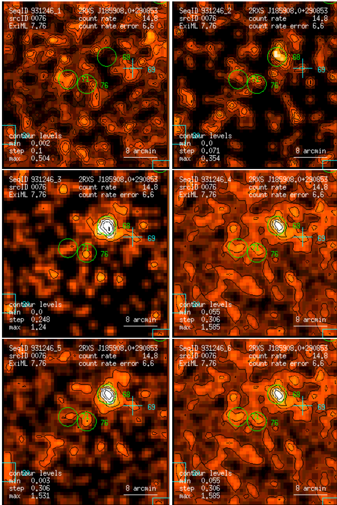
Figure 76: RASS 931246: detection 0076: band rate images, Gaussian filter: (1) PSPC channels 11 – 41, (2) 52 – 90, (3) 91 – 201, (4) 11 – 235, (5) 52 – 201, (6) 11 – 201. Broad band rates in counts/ks. Band rate contour levels in counts/ks/arcmin 2 .
