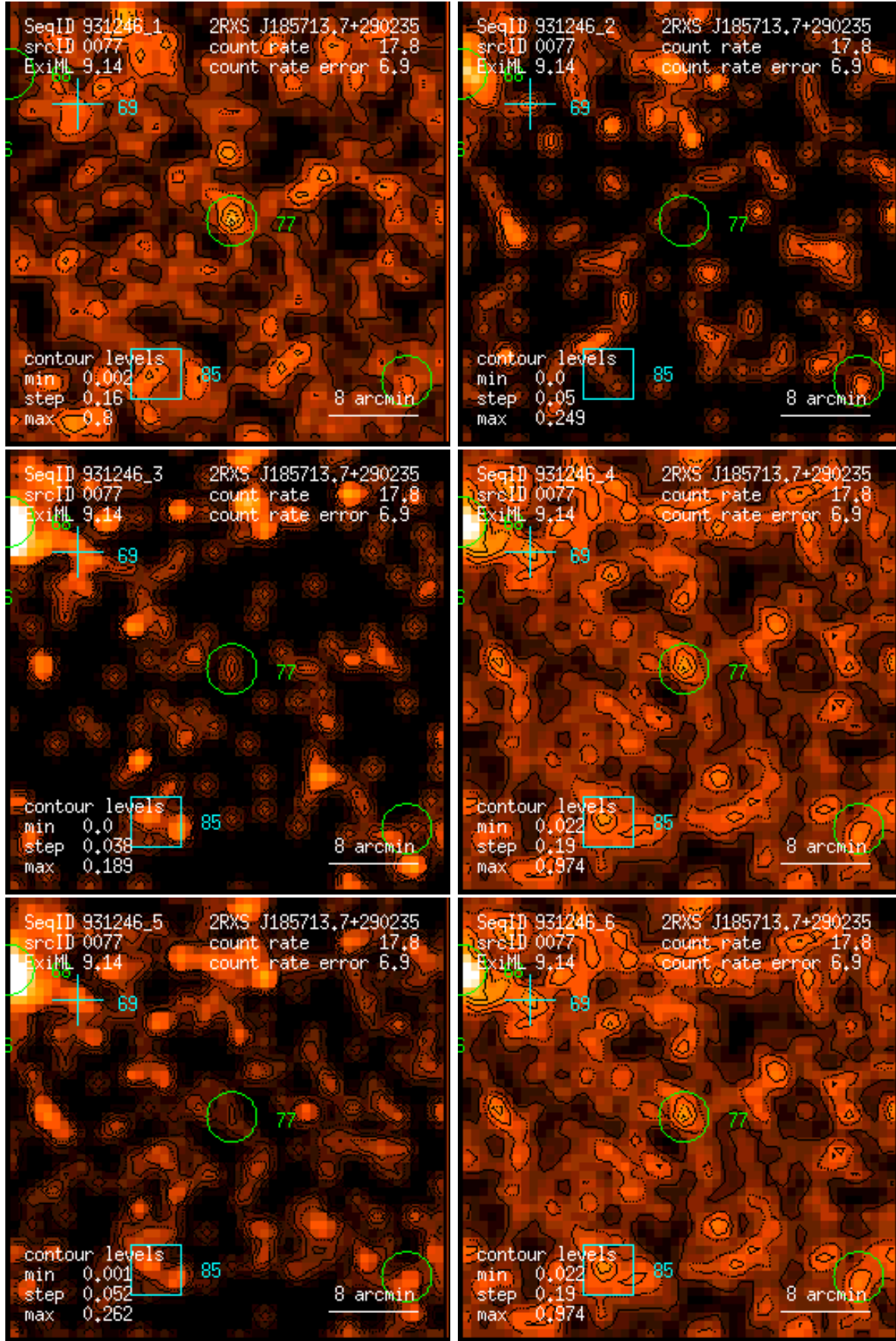
Figure 77: RASS 931246: detection 0077: band rate images, Gaussian filter: (1) PSPC channels 11 – 41, (2) 52 – 90, (3) 91 – 201, (4) 11 – 235, (5) 52 – 201, (6) 11 – 201. Broad band rates in counts/ks. Band rate contour levels in counts/ks/arcmin 2 .
