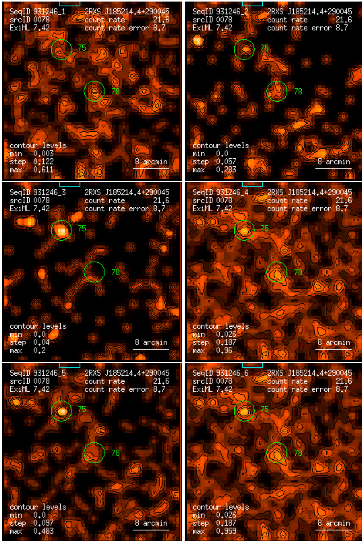
Figure 78: RASS 931246: detection 0078: band rate images, Gaussian filter: (1) PSPC channels 11 – 41, (2) 52 – 90, (3) 91 – 201, (4) 11 – 235, (5) 52 – 201, (6) 11 – 201. Broad band rates in counts/ks. Band rate contour levels in counts/ks/arcmin 2 .
