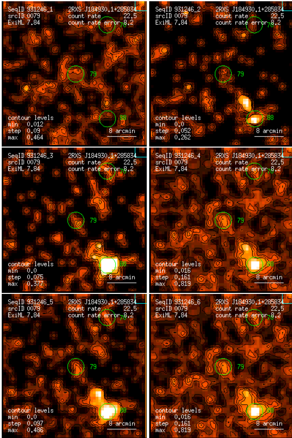
Figure 79: RASS 931246: detection 0079: band rate images, Gaussian filter: (1) PSPC channels 11 – 41, (2) 52 – 90, (3) 91 – 201, (4) 11 – 235, (5) 52 – 201, (6) 11 – 201. Broad band rates in counts/ks. Band rate contour levels in counts/ks/arcmin 2 .
