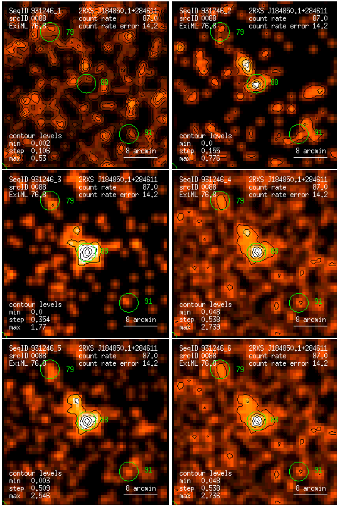
Figure 88: RASS 931246: detection 0088: band rate images, Gaussian filter: (1) PSPC channels 11 – 41, (2) 52 – 90, (3) 91 – 201, (4) 11 – 235, (5) 52 – 201, (6) 11 – 201. Broad band rates in counts/ks. Band rate contour levels in counts/ks/arcmin 2 .
