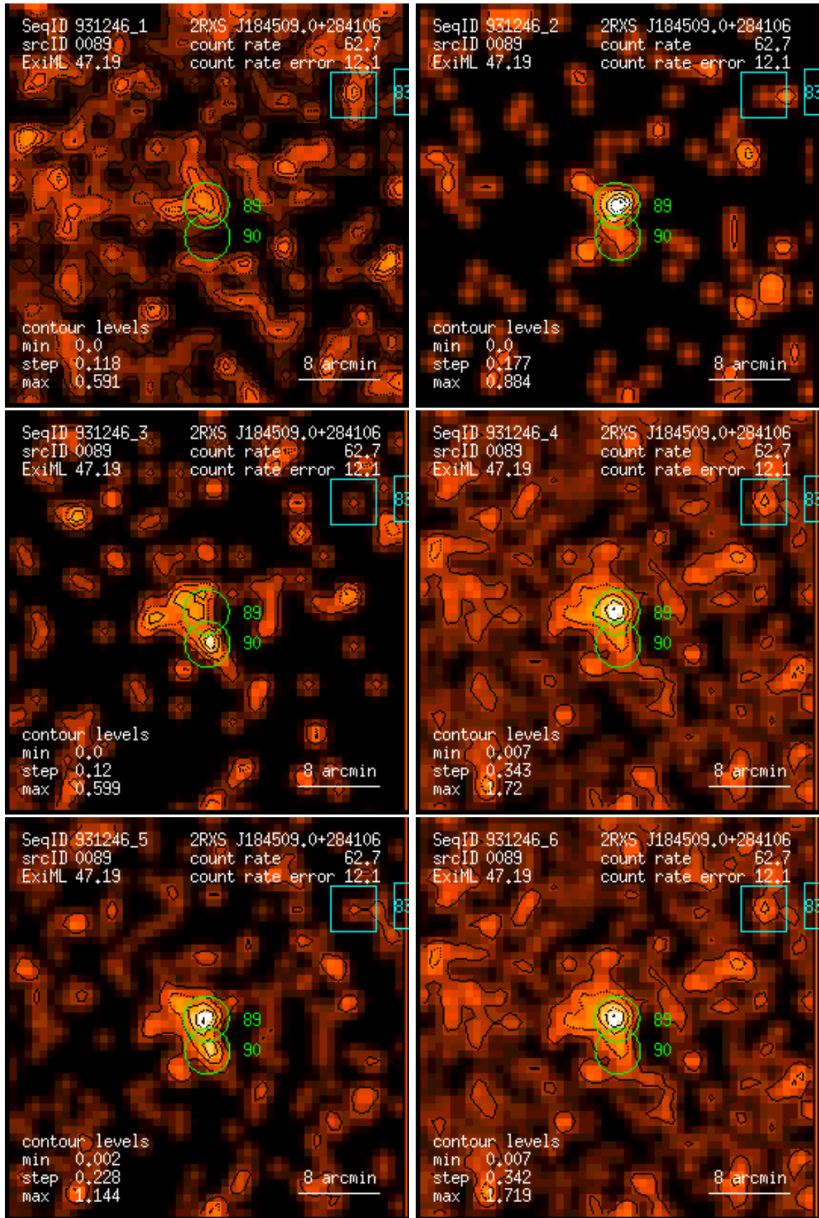
Figure 89: RASS 931246: detection 0089: band rate images, Gaussian filter: (1) PSPC channels 11 – 41, (2) 52 – 90, (3) 91 – 201, (4) 11 – 235, (5) 52 – 201, (6) 11 – 201. Broad band rates in counts/ks. Band rate contour levels in counts/ks/arcmin 2 .
