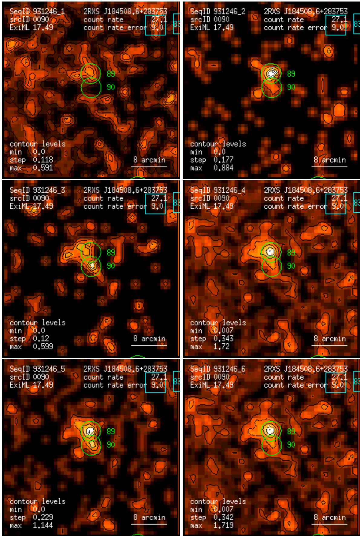
Figure 90: RASS 931246: detection 0090: band rate images, Gaussian filter: (1) PSPC channels 11 – 41, (2) 52 – 90, (3) 91 – 201, (4) 11 – 235, (5) 52 – 201, (6) 11 – 201. Broad band rates in counts/ks. Band rate contour levels in counts/ks/arcmin 2 .
