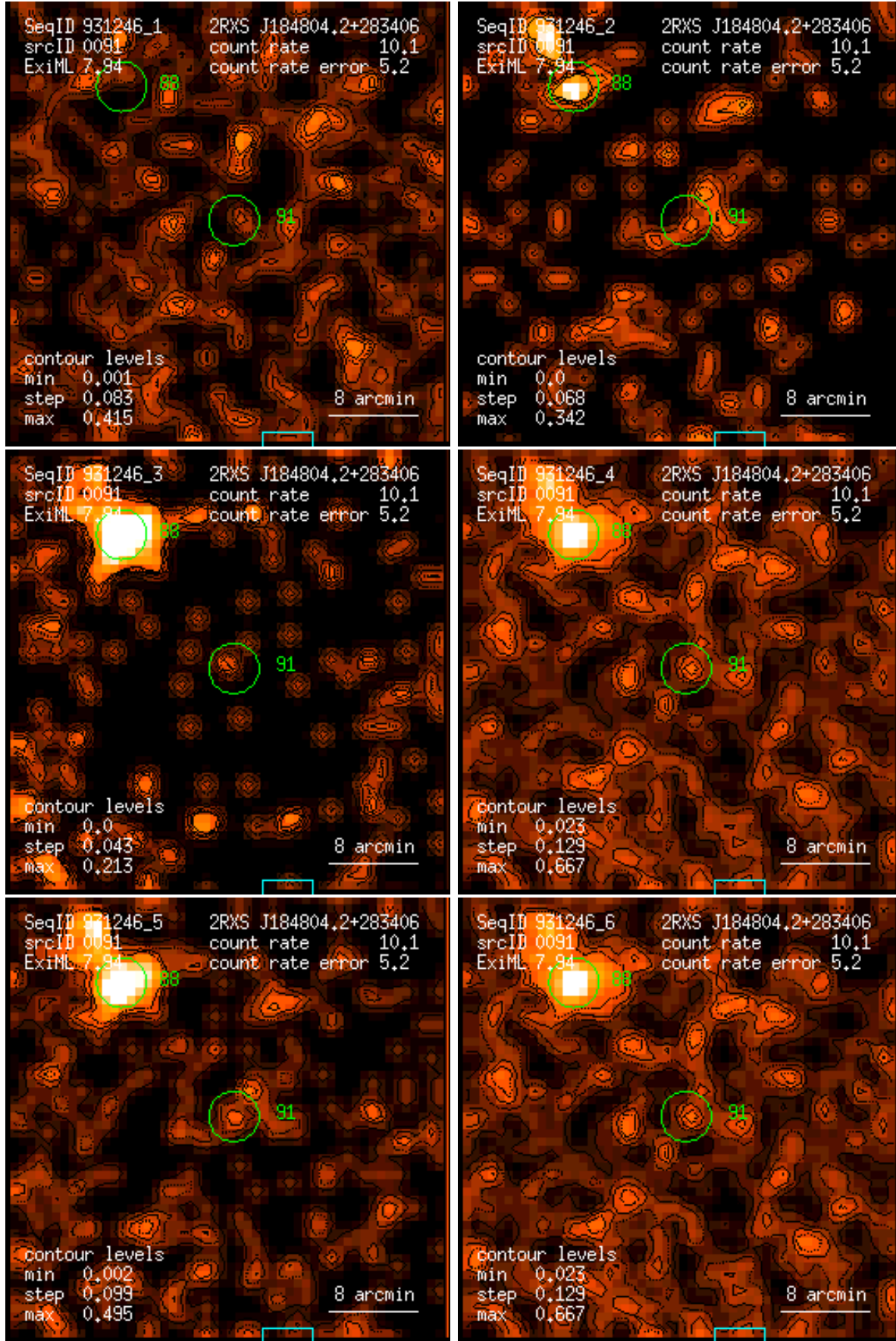
Figure 91: RASS 931246: detection 0091: band rate images, Gaussian filter: (1) PSPC channels 11 – 41, (2) 52 – 90, (3) 91 – 201, (4) 11 – 235, (5) 52 – 201, (6) 11 – 201. Broad band rates in counts/ks. Band rate contour levels in counts/ks/arcmin 2 .
