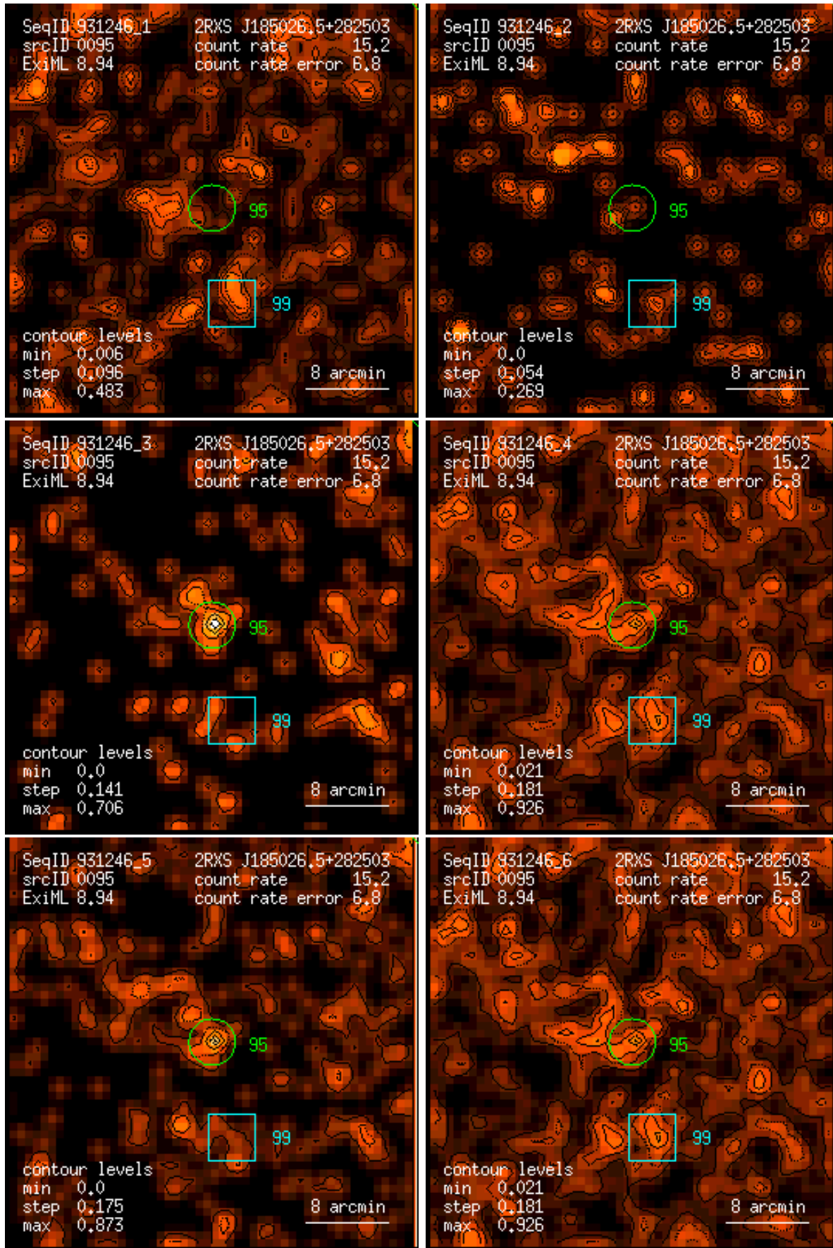
Figure 95: RASS 931246: detection 0095: band rate images, Gaussian filter: (1) PSPC channels 11 – 41, (2) 52 – 90, (3) 91 – 201, (4) 11 – 235, (5) 52 – 201, (6) 11 – 201. Broad band rates in counts/ks. Band rate contour levels in counts/ks/arcmin 2 .
