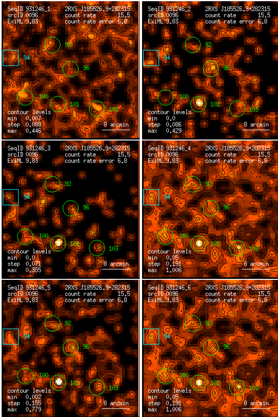
Figure 96: RASS 931246: detection 0096: band rate images, Gaussian filter: (1) PSPC channels 11 – 41, (2) 52 – 90, (3) 91 – 201, (4) 11 – 235, (5) 52 – 201, (6) 11 – 201. Broad band rates in counts/ks. Band rate contour levels in counts/ks/arcmin 2 .
