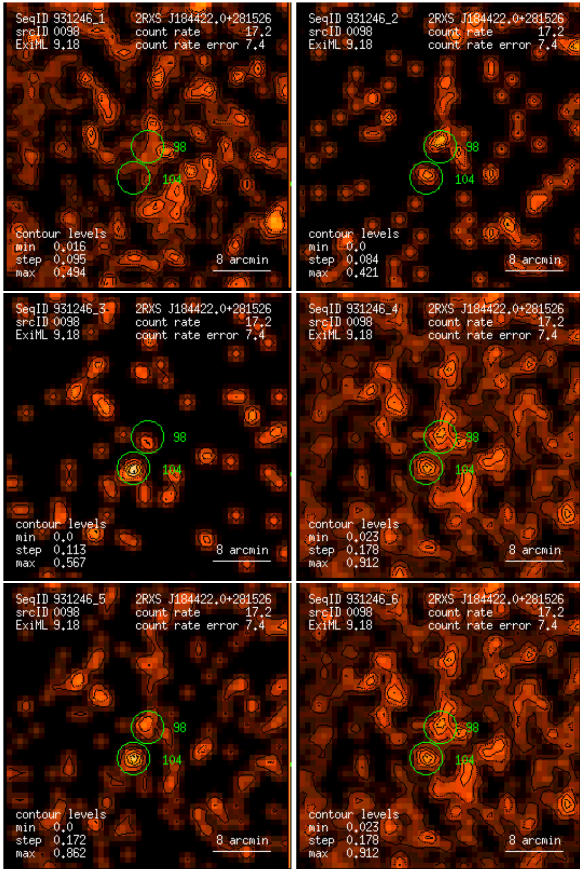
Figure 98: RASS 931246: detection 0098: band rate images, Gaussian filter: (1) PSPC channels 11 – 41, (2) 52 – 90, (3) 91 – 201, (4) 11 – 235, (5) 52 – 201, (6) 11 – 201. Broad band rates in counts/ks. Band rate contour levels in counts/ks/arcmin 2 .
