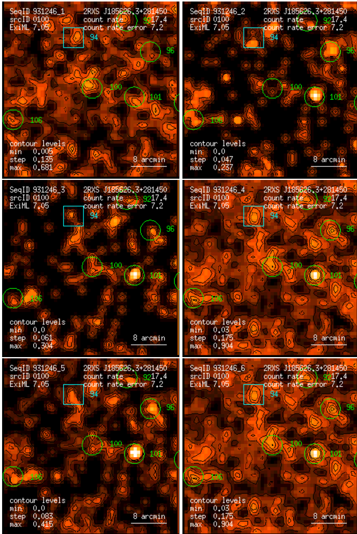
Figure 100: RASS 931246: detection 0100: band rate images, Gaussian filter: (1) PSPC channels 11 – 41, (2) 52 – 90, (3) 91 – 201, (4) 11 – 235, (5) 52 – 201, (6) 11 – 201. Broad band rates in counts/ks. Band rate contour levels in counts/ks/arcmin 2 .
