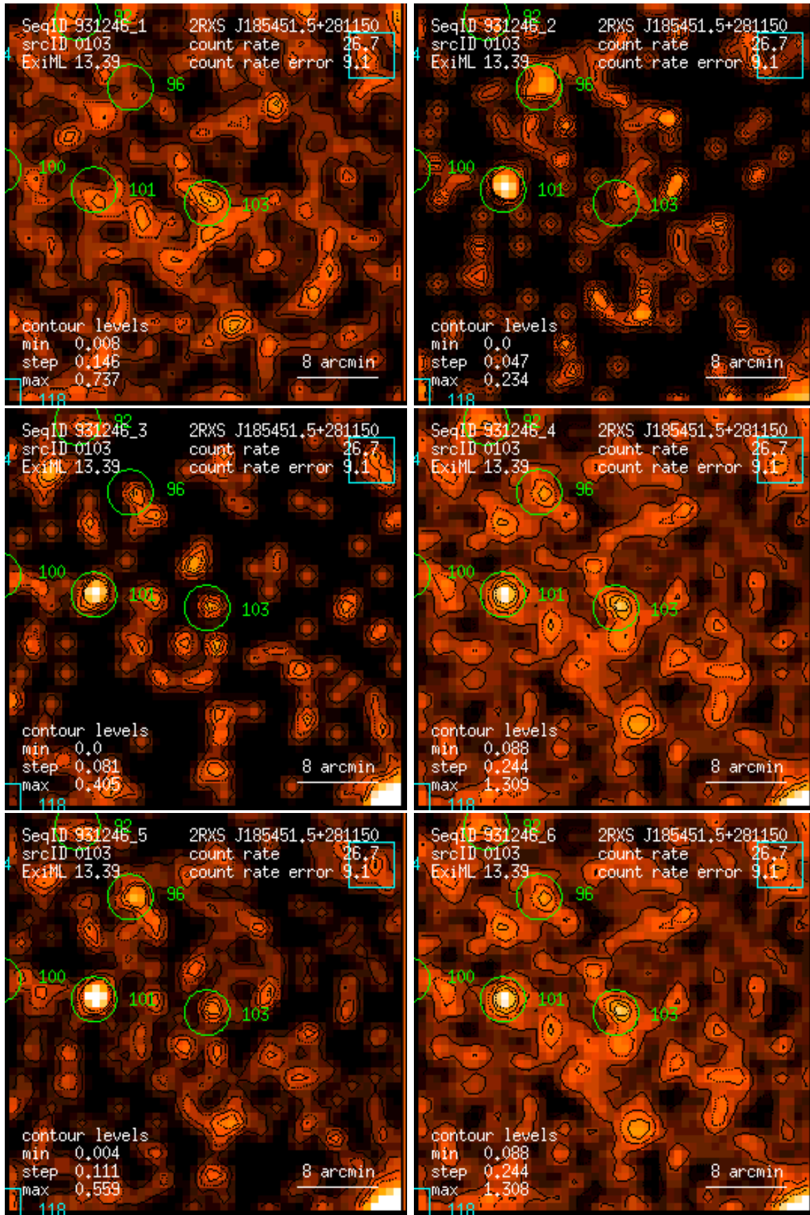
Figure 103: RASS 931246: detection 0103: band rate images, Gaussian filter: (1) PSPC channels 11 – 41, (2) 52 – 90, (3) 91 – 201, (4) 11 – 235, (5) 52 – 201, (6) 11 – 201. Broad band rates in counts/ks. Band rate contour levels in counts/ks/arcmin 2 .
