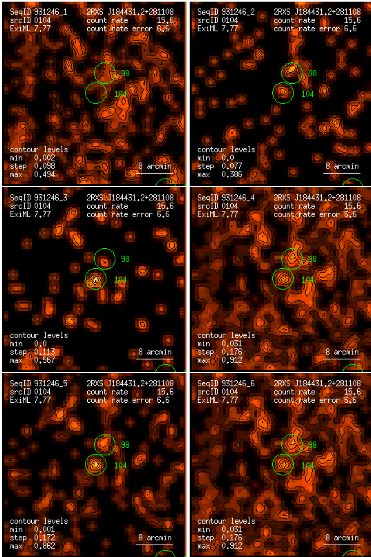
Figure 104: RASS 931246: detection 0104: band rate images, Gaussian filter: (1) PSPPC channels 11 – 41, (2) 52 – 90, (3) 91 – 201, (4) 11 – 235, (5) 52 – 201, (6) 11 – 201. Broad band rates in counts/ks. Band rate contour levels in counts/ks/arcmin 2 .
