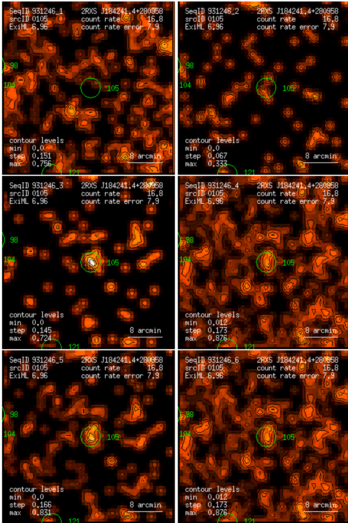
Figure 105: RASS 931246: detection 0105: band rate images, Gaussian filter: (1) PSPC channels 11 – 41, (2) 52 – 90, (3) 91 – 201, (4) 11 – 235, (5) 52 – 201, (6) 11 – 201. Broad band rates in counts/ks. Band rate contour levels in counts/ks/arcmin 2 .
