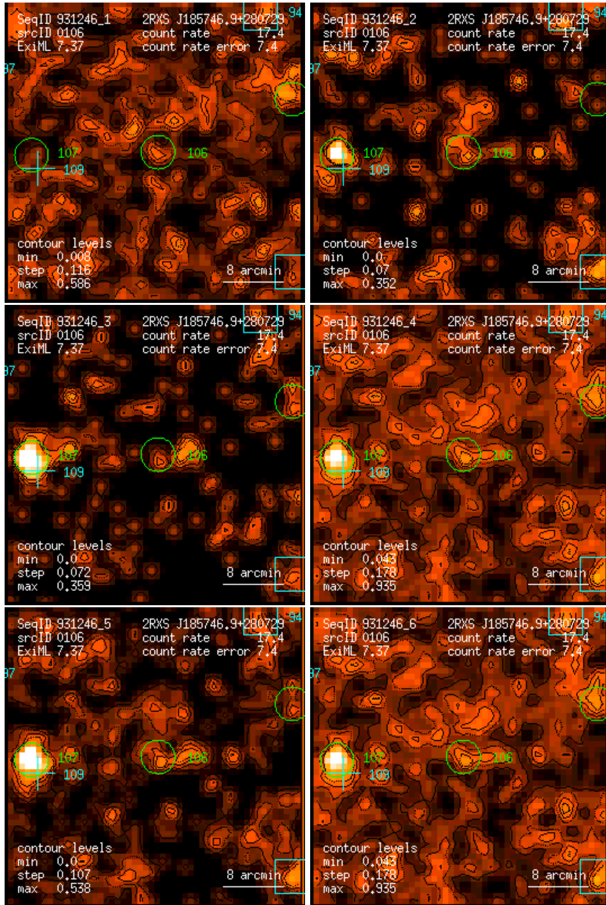
Figure 106: RASS 931246: detection 0106: band rate images, Gaussian filter: (1) PSPC channels 11 – 41, (2) 52 – 90, (3) 91 – 201, (4) 11 – 235, (5) 52 – 201, (6) 11 – 201. Broad band rates in counts/ks. Band rate contour levels in counts/ks/arcmin 2 .
