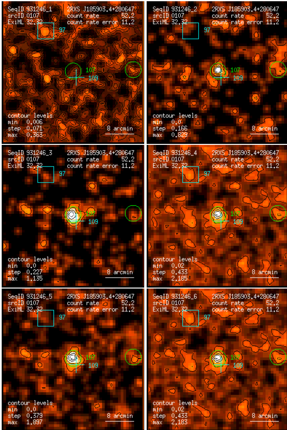
Figure 107: RASS 931246: detection 0107: band rate images, Gaussian filter: (1) PSPC channels 11 – 41, (2) 52 – 90, (3) 91 – 201, (4) 11 – 235, (5) 52 – 201, (6) 11 – 201. Broad band rates in counts/ks. Band rate contour levels in counts/ks/arcmin 2 .
