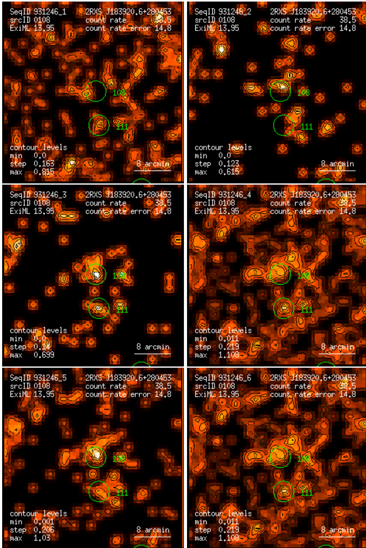
Figure 108: RASS 931246: detection 0108: band rate images, Gaussian filter: (1) PSPPC channels 11 – 41, (2) 52 – 90, (3) 91 – 201, (4) 11 – 235, (5) 52 – 201, (6) 11 – 201. Broad band rates in counts/ks. Band rate contour levels in counts/ks/arcmin 2 .
