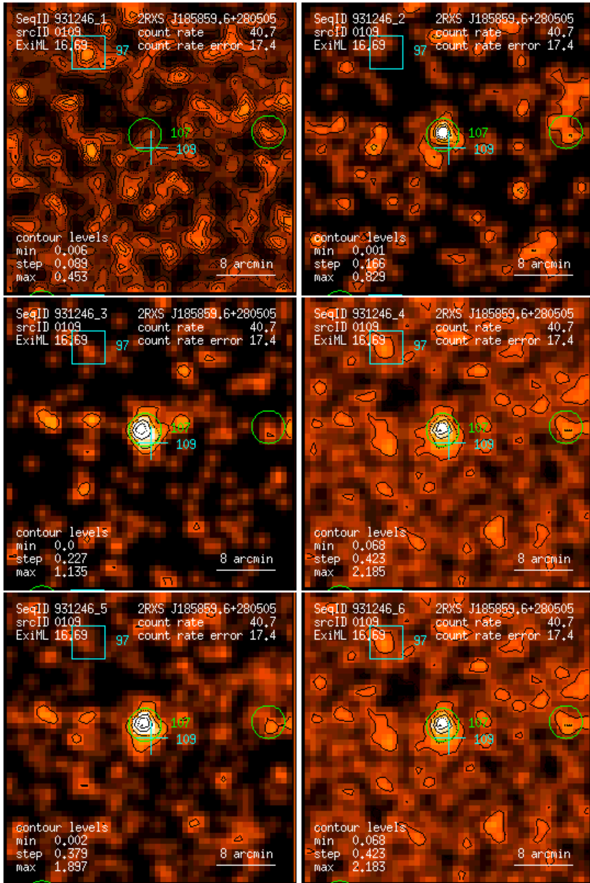
Figure 109: RASS 931246: detection 0109: band rate images, Gaussian filter: (1) PSPC channels 11 – 41, (2) 52 – 90, (3) 91 – 201, (4) 11 – 235, (5) 52 – 201, (6) 11 – 201. Broad band rates in counts/ks. Band rate contour levels in counts/ks/arcmin 2 .
