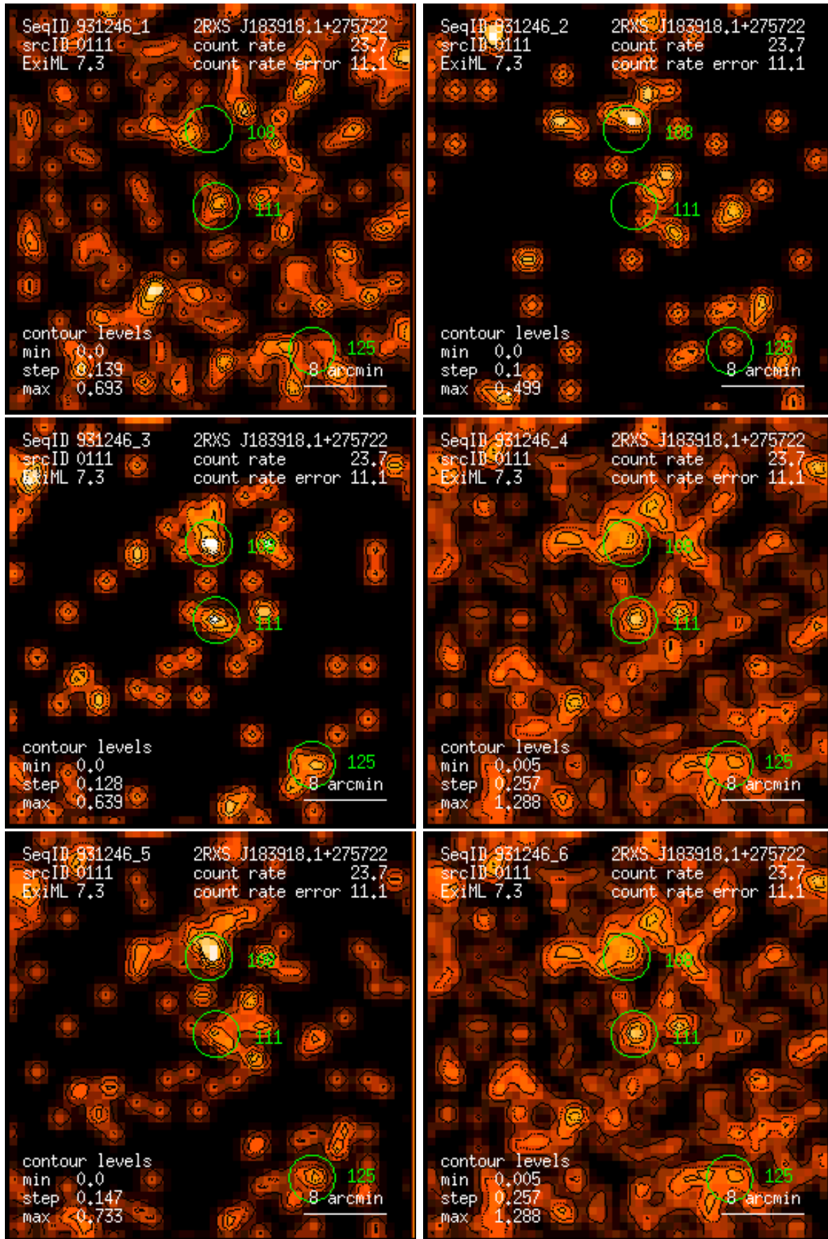
Figure 111: RASS 931246: detection 0111: band rate images, Gaussian filter: (1) PSPP channels 11 – 41, (2) 52 – 90, (3) 91 – 201, (4) 11 – 235, (5) 52 – 201, (6) 11 – 201. Broad band rates in counts/ks. Band rate contour levels in counts/ks/arcmin 2 .
