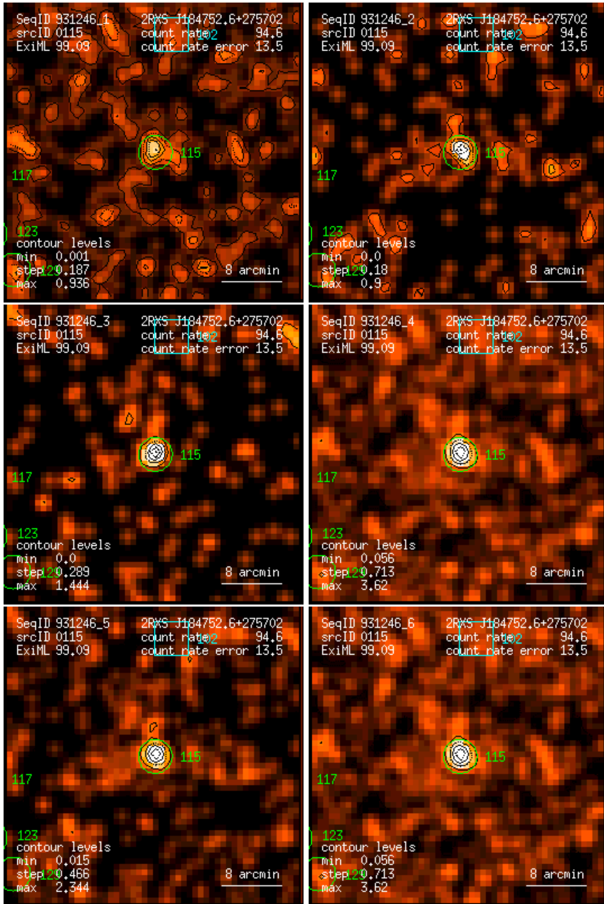
Figure 115: RASS 931246: detection 0115: band rate images, Gaussian filter: (1) PSPC channels 11 – 41, (2) 52 – 90, (3) 91 – 201, (4) 11 – 235, (5) 52 – 201, (6) 11 – 201. Broad band rates in counts/ks. Band rate contour levels in counts/ks/arcmin 2 .
