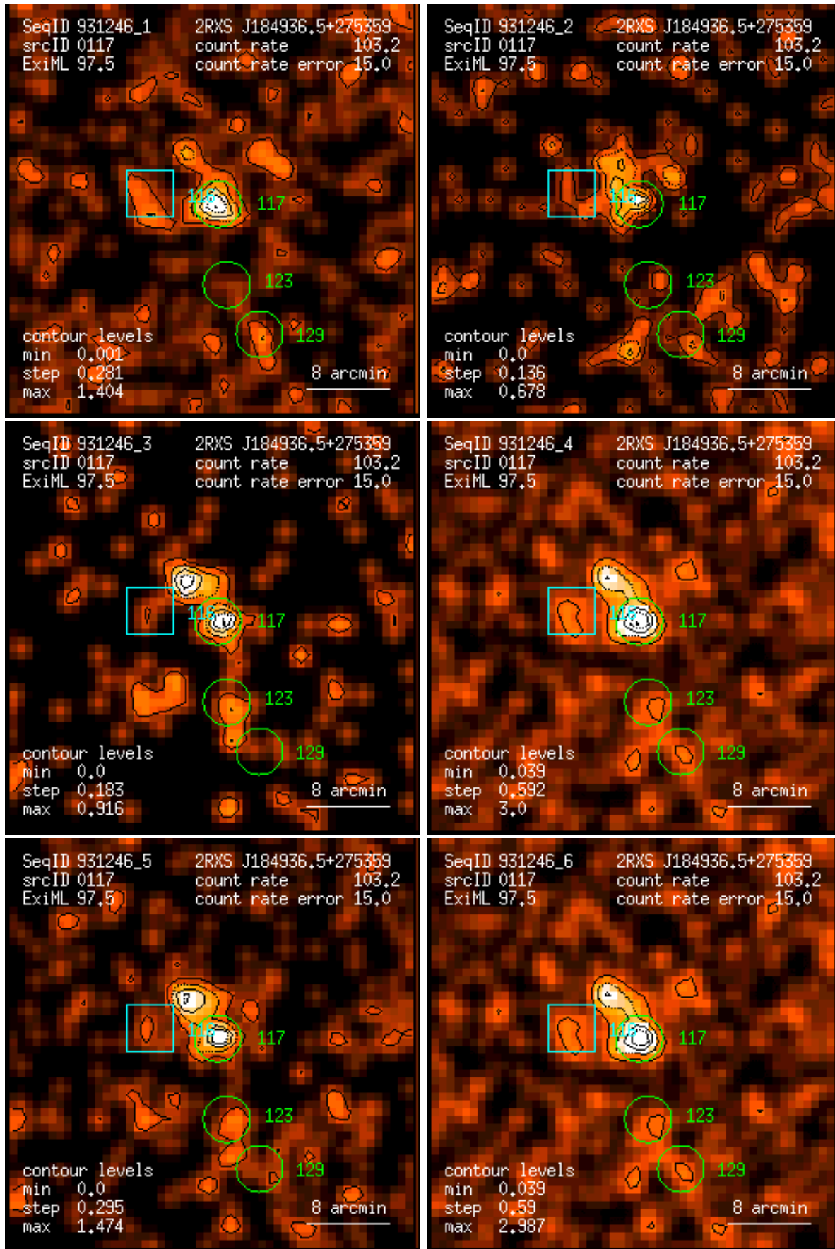
Figure 117: RASS 931246: detection 0117: band rate images, Gaussian filter: (1) PSPC channels 11 – 41, (2) 52 – 90, (3) 91 – 201, (4) 11 – 235, (5) 52 – 201, (6) 11 – 201. Broad band rates in counts/ks. Band rate contour levels in counts/ks/arcmin 2 .
