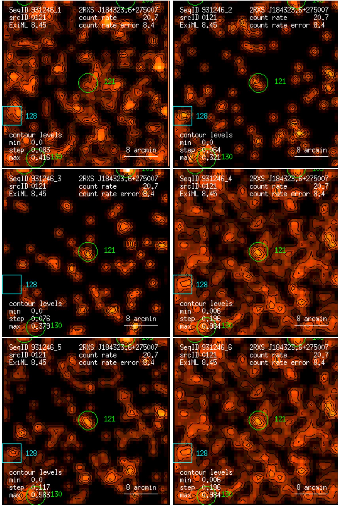
Figure 121: RASS 931246: detection 0121: band rate images, Gaussian filter: (1) PSPC channels 11 – 41, (2) 52 – 90, (3) 91 – 201, (4) 11 – 235, (5) 52 – 201, (6) 11 – 201. Broad band rates in counts/ks. Band rate contour levels in counts/ks/arcmin 2 .
