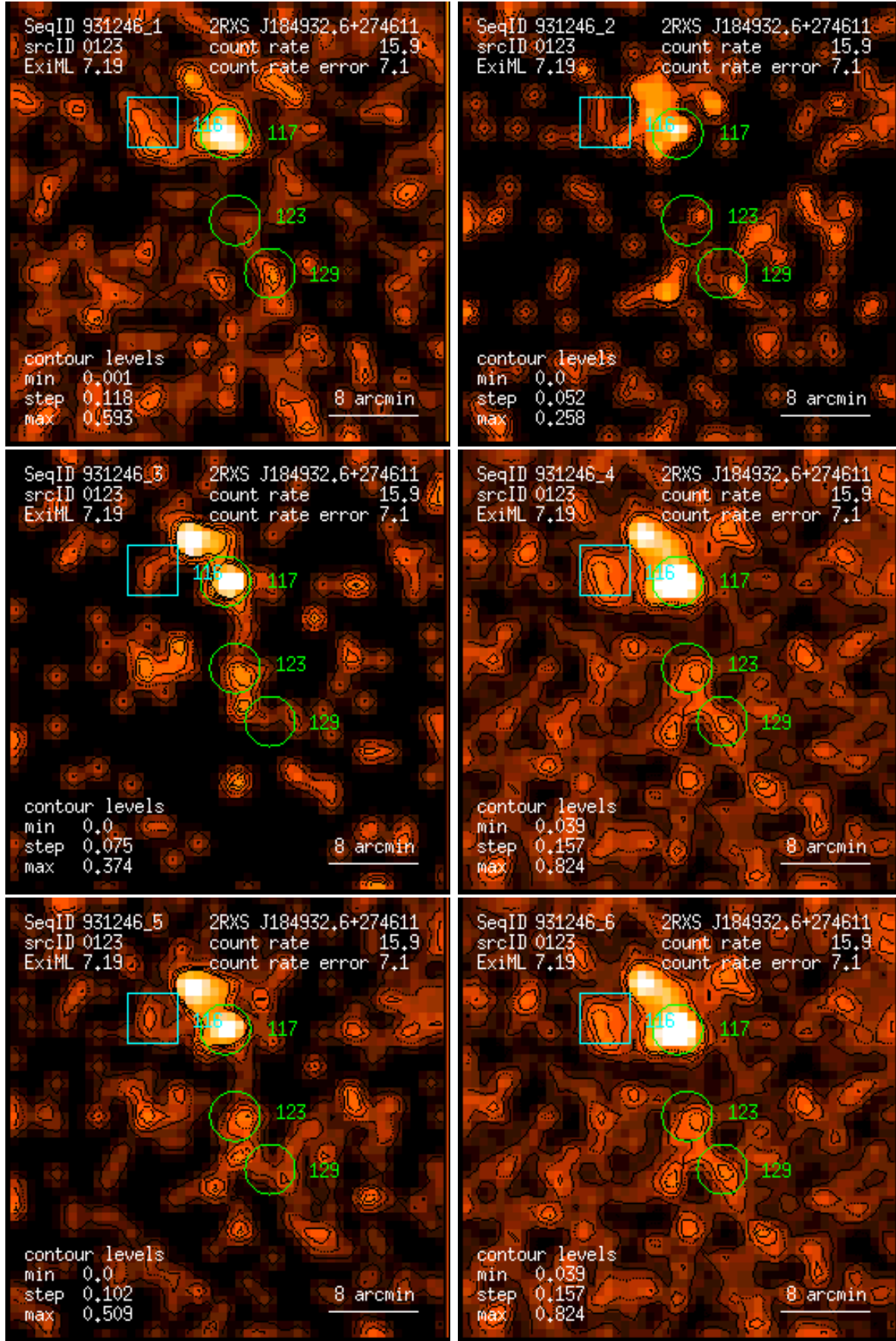
Figure 123: RASS 931246: detection 0123: band rate images, Gaussian filter: (1) PSPC channels 11 – 41, (2) 52 – 90, (3) 91 – 201, (4) 11 – 235, (5) 52 – 201, (6) 11 – 201. Broad band rates in counts/ks. Band rate contour levels in counts/ks/arcmin 2 .
