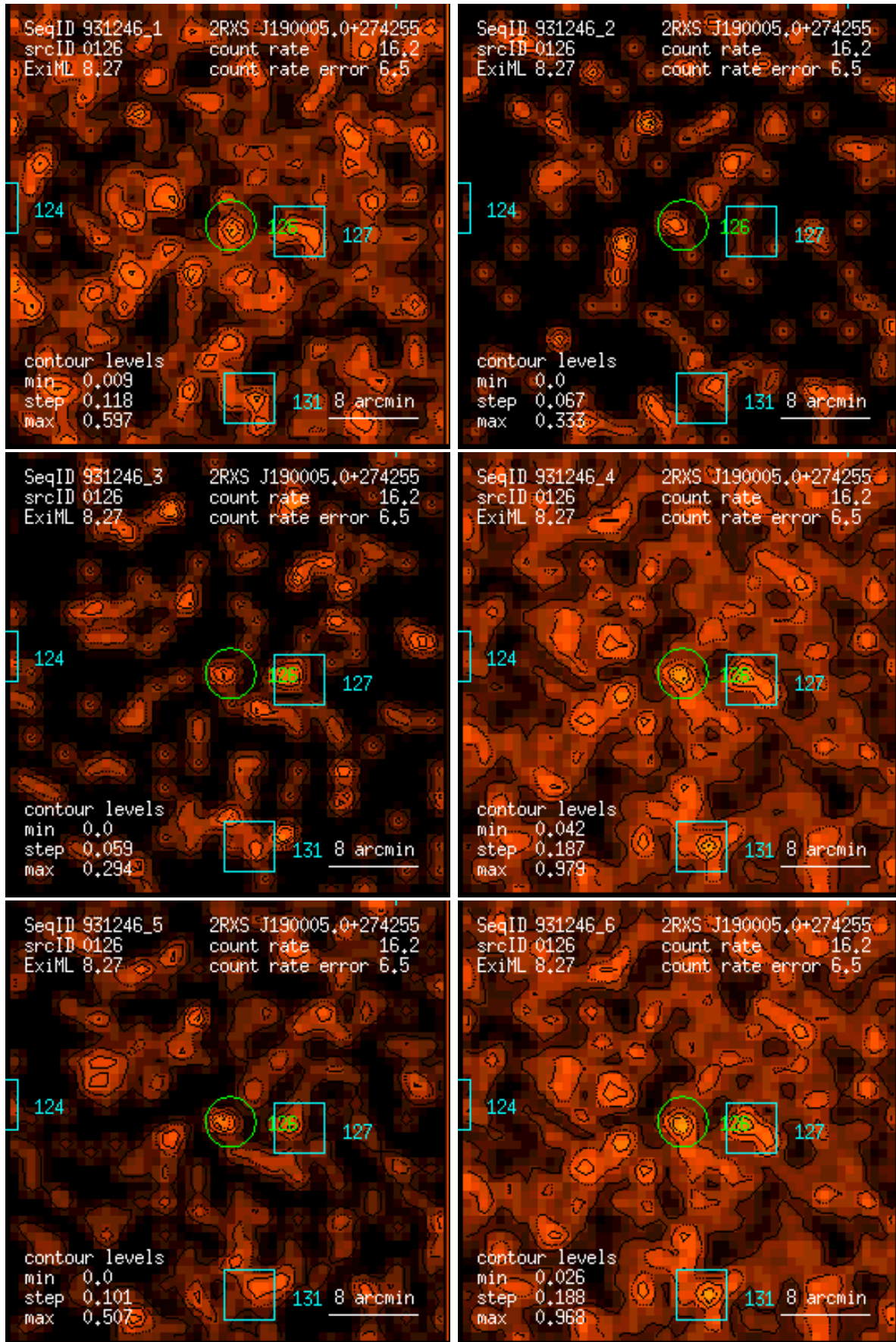
Figure 126: RASS 931246: detection 0126: band rate images, Gaussian filter: (1) PSPC channels 11 – 41, (2) 52 – 90, (3) 91 – 201, (4) 11 – 235, (5) 52 – 201, (6) 11 – 201. Broad band rates in counts/ks. Band rate contour levels in counts/ks/arcmin 2 .
