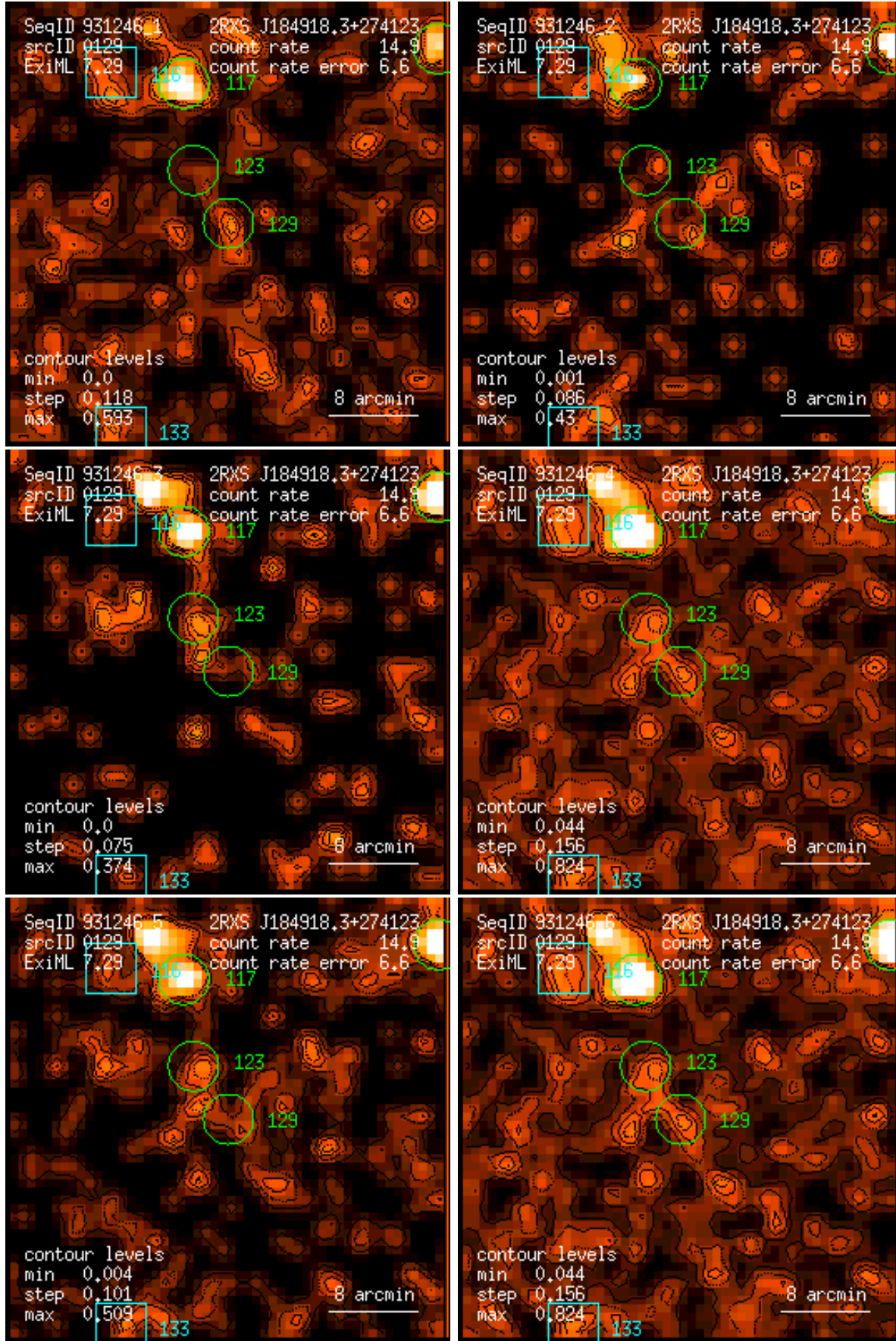
Figure 129: RASS 931246: detection 0129: band rate images, Gaussian filter: (1) PSPC channels 11 – 41, (2) 52 – 90, (3) 91 – 201, (4) 11 – 235, (5) 52 – 201, (6) 11 – 201. Broad band rates in counts/ks. Band rate contour levels in counts/ks/arcmin 2 .
