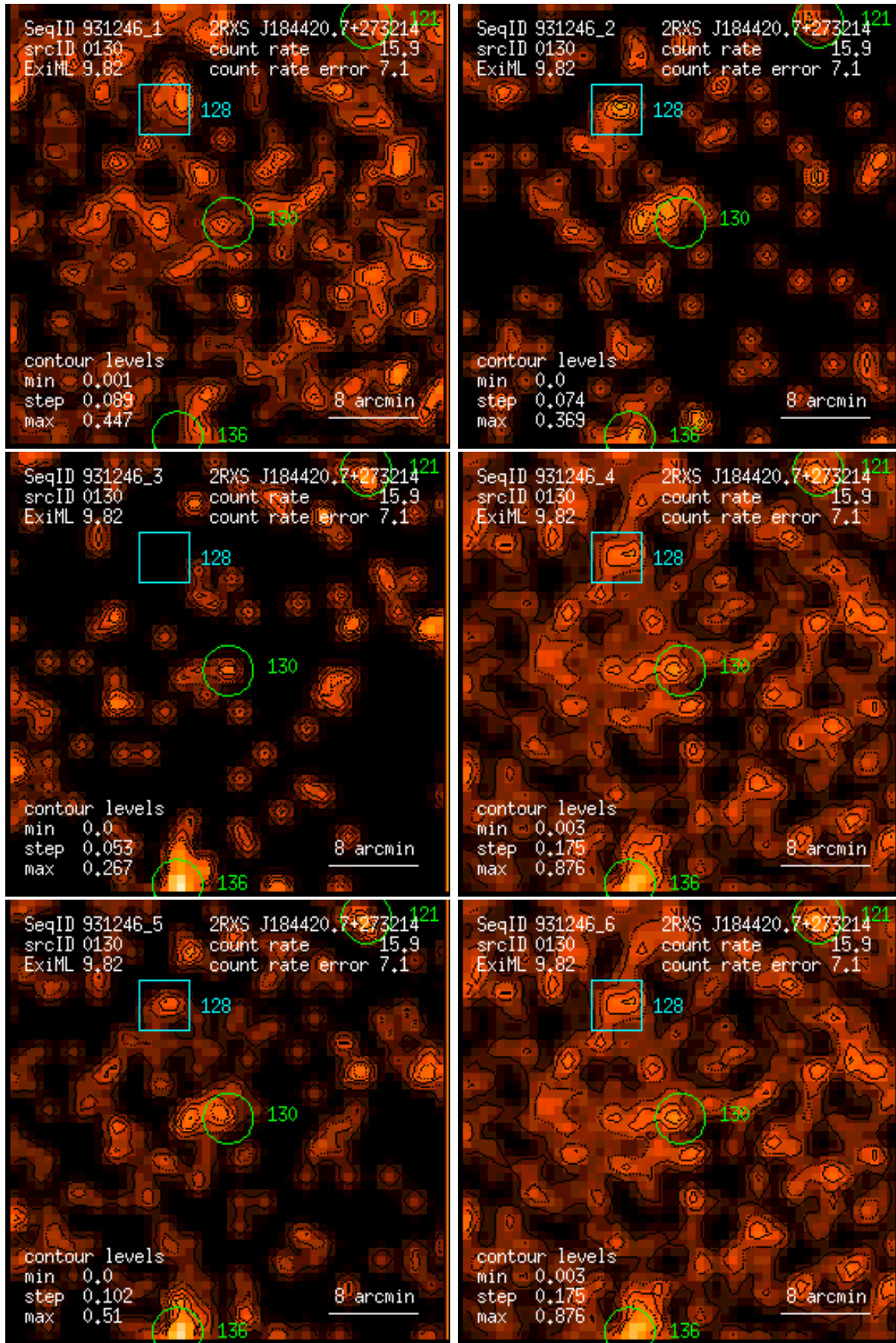
Figure 130: RASS 931246: detection 0130: band rate images, Gaussian filter: (1) PSPC channels 11 – 41, (2) 52 – 90, (3) 91 – 201, (4) 11 – 235, (5) 52 – 201, (6) 11 – 201. Broad band rates in counts/ks. Band rate contour levels in counts/ks/arcmin 2 .
