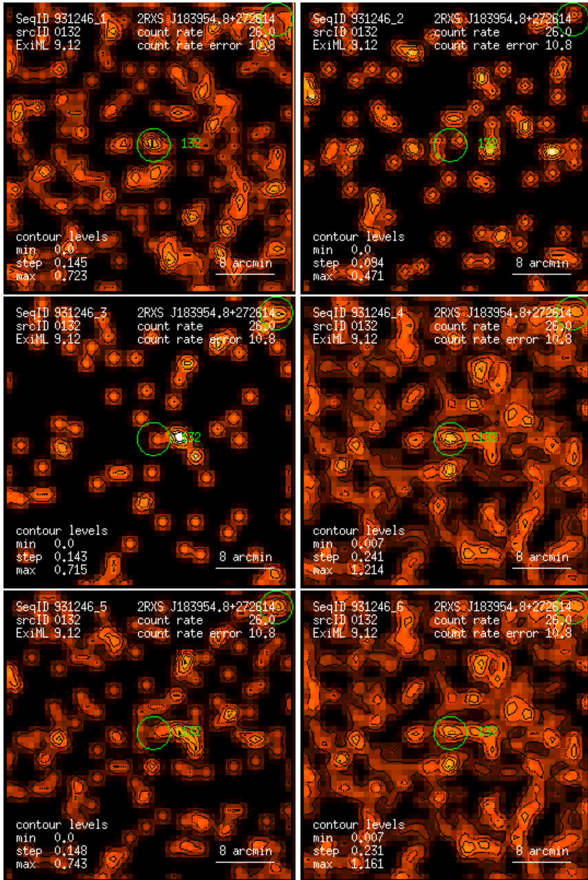
Figure 132: RASS 931246: detection 0132: band rate images, Gaussian filter: (1) PSPC channels 11 – 41, (2) 52 – 90, (3) 91 – 201, (4) 11 – 235, (5) 52 – 201, (6) 11 – 201. Broad band rates in counts/ks. Band rate contour levels in counts/ks/arcmin 2 .
