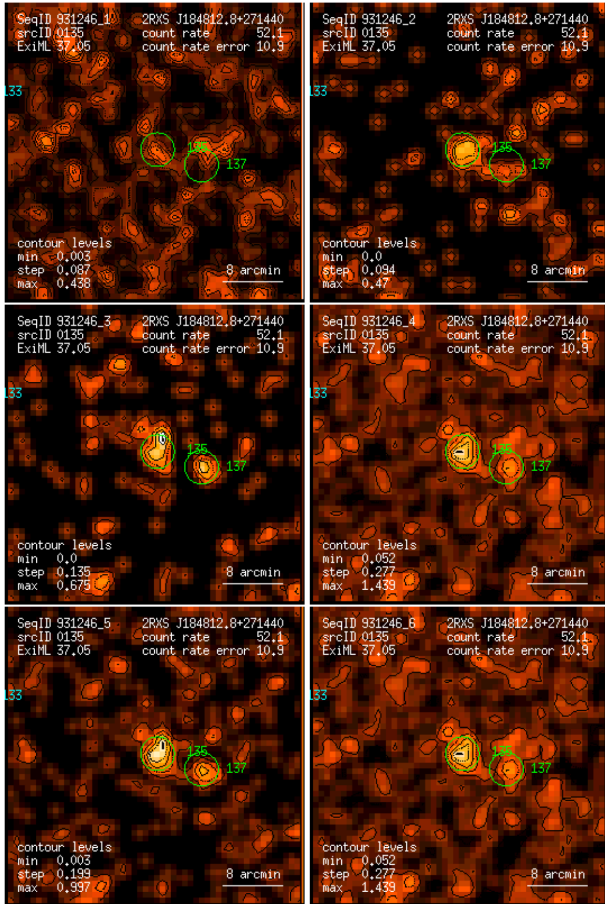
Figure 135: RASS 931246: detection 0135: band rate images, Gaussian filter: (1) PSPC channels 11 – 41, (2) 52 – 90, (3) 91 – 201, (4) 11 – 235, (5) 52 – 201, (6) 11 – 201. Broad band rates in counts/ks. Band rate contour levels in counts/ks/arcmin 2 .
