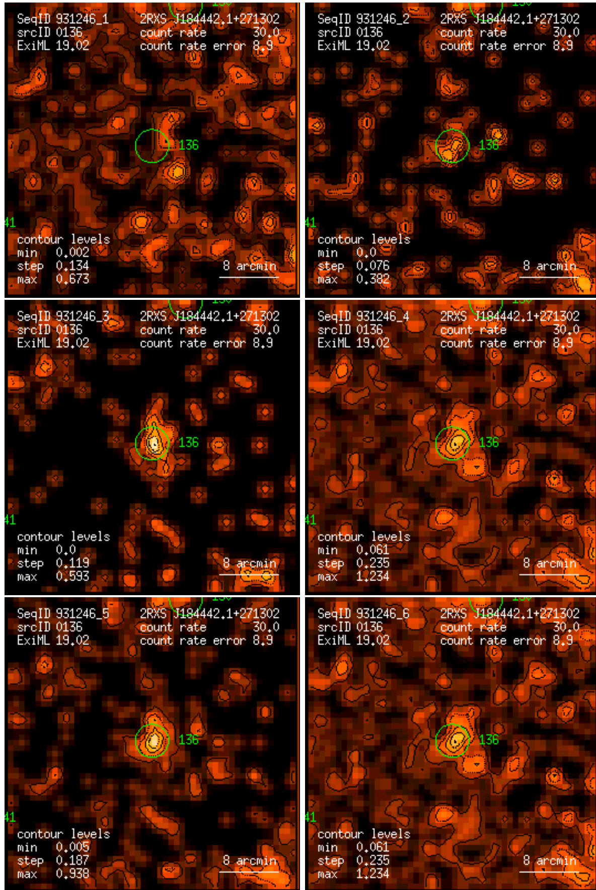
Figure 136: RASS 931246: detection 0136: band rate images, Gaussian filter: (1) PSPC channels 11 – 41, (2) 52 – 90, (3) 91 – 201, (4) 11 – 235, (5) 52 – 201, (6) 11 – 201. Broad band rates in counts/ks. Band rate contour levels in counts/ks/arcmin 2 .
