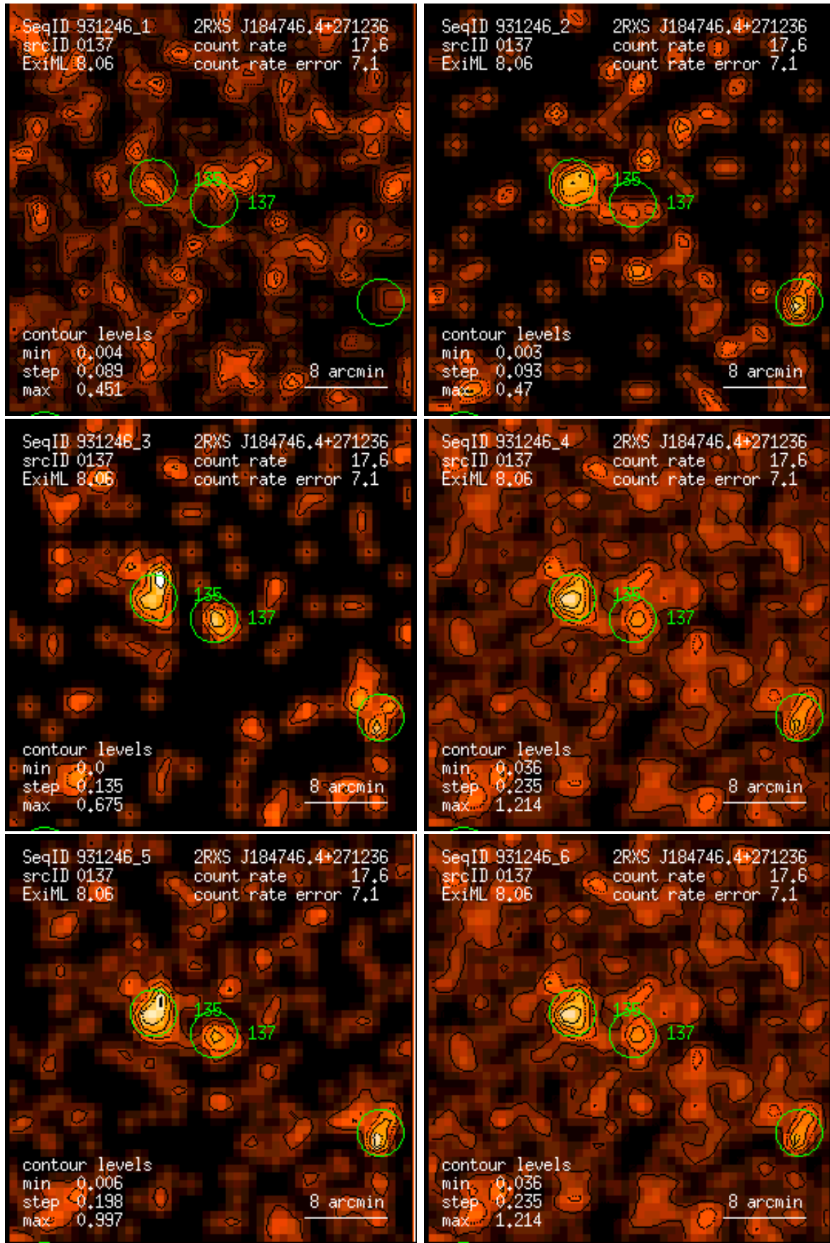
Figure 137: RASS 931246: detection 0137: band rate images, Gaussian filter: (1) PSPC channels 11 – 41, (2) 52 – 90, (3) 91 – 201, (4) 11 – 235, (5) 52 – 201, (6) 11 – 201. Broad band rates in counts/ks. Band rate contour levels in counts/ks/arcmin 2 .
