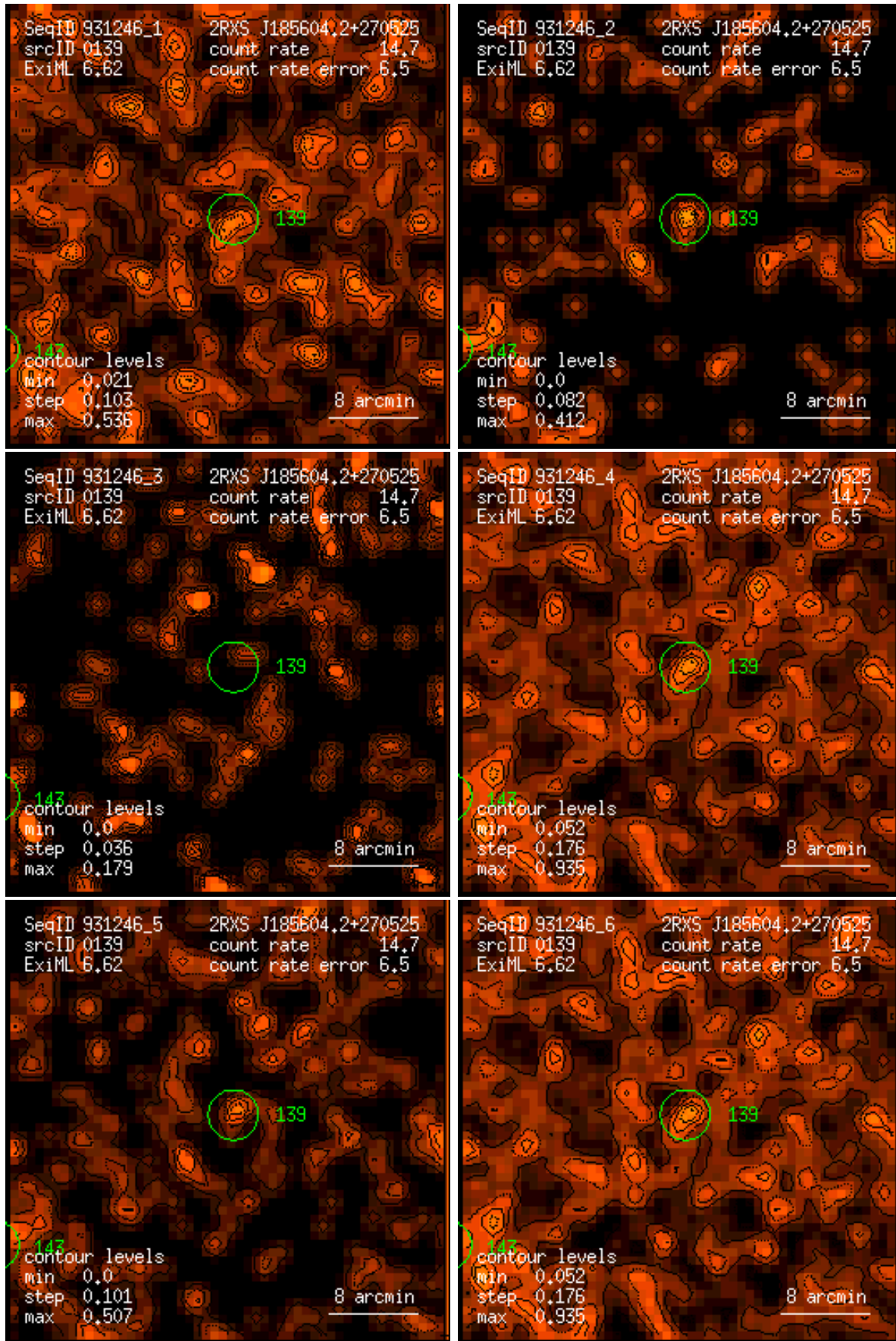
Figure 139: RASS 931246: detection 0139: band rate images, Gaussian filter: (1) PSPC channels 11 – 41, (2) 52 – 90, (3) 91 – 201, (4) 11 – 235, (5) 52 – 201, (6) 11 – 201. Broad band rates in counts/ks. Band rate contour levels in counts/ks/arcmin 2 .
