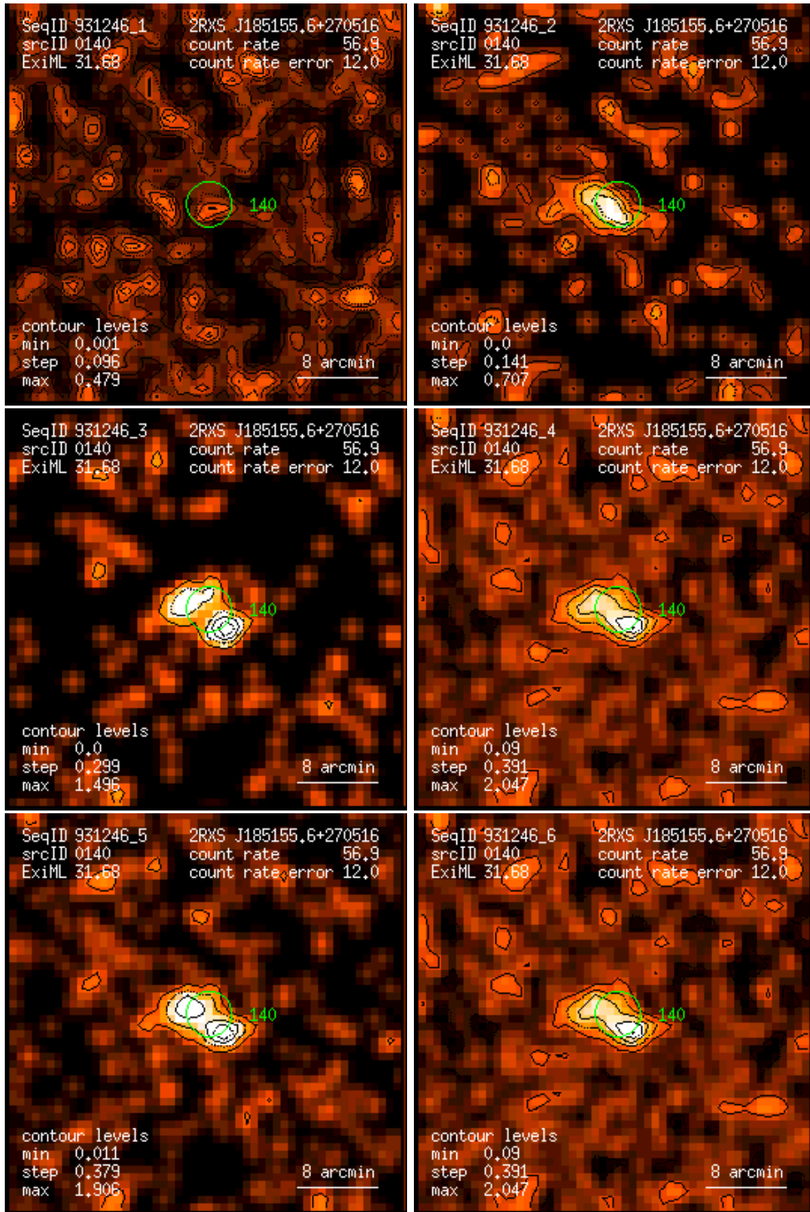
Figure 140: RASS 931246: detection 0140: band rate images, Gaussian filter: (1) PSPC channels 11 – 41, (2) 52 – 90, (3) 91 – 201, (4) 11 – 235, (5) 52 – 201, (6) 11 – 201. Broad band rates in counts/ks. Band rate contour levels in counts/ks/arcmin 2 .
