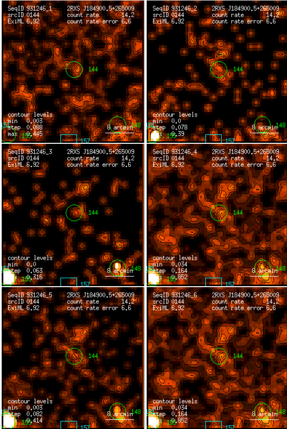
Figure 144: RASS 931246: detection 0144: band rate images, Gaussian filter: (1) PSPC channels 11 – 41, (2) 52 – 90, (3) 91 – 201, (4) 11 – 235, (5) 52 – 201, (6) 11 – 201. Broad band rates in counts/ks. Band rate contour levels in counts/ks/arcmin 2 .
